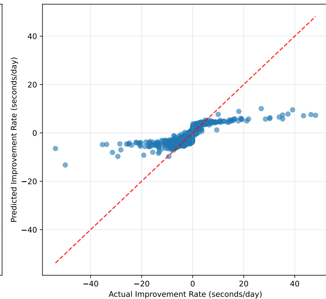
SVR R^2 = 0.5140
