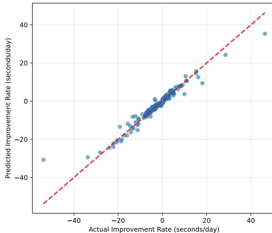
Gradient Boosting R^2 = 0.934 (95% CI: [0.894, 0.967]) n=348
