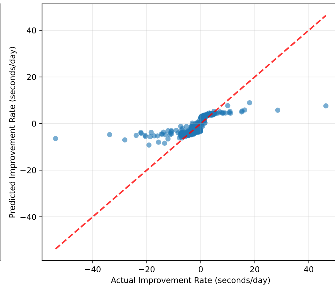
SVR R^2 = 0.537 (95% CI: [0.441, 0.661]) n=348
