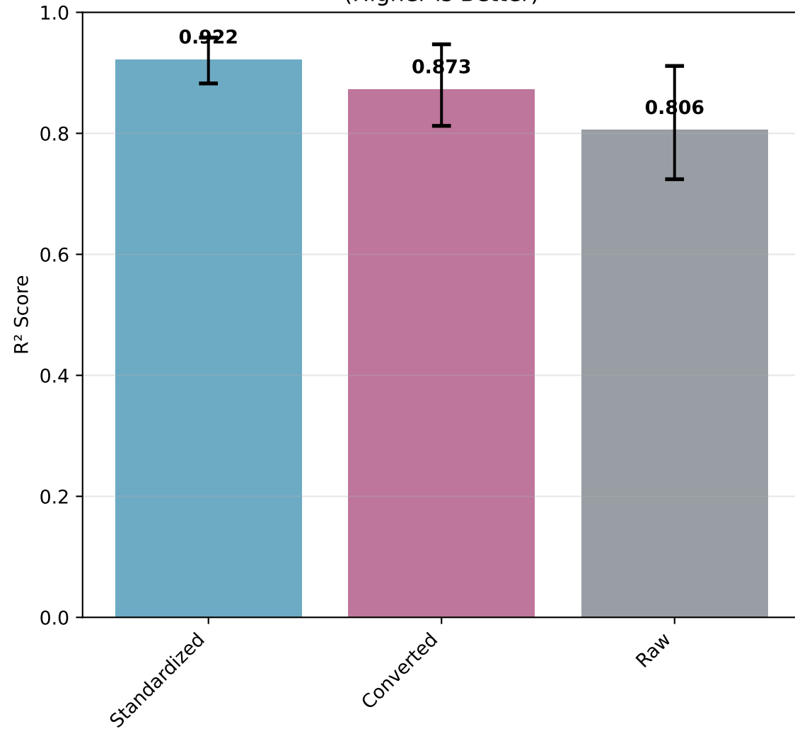
Model Performance by Time Standardization Method (Higher is Better)
