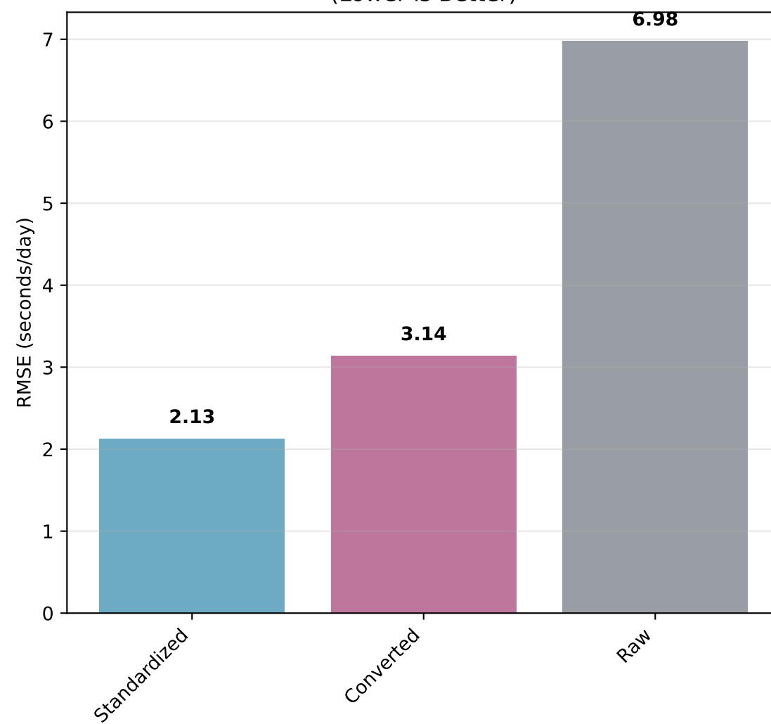
RMSE by Time Standardization Method (Lower is Better)
