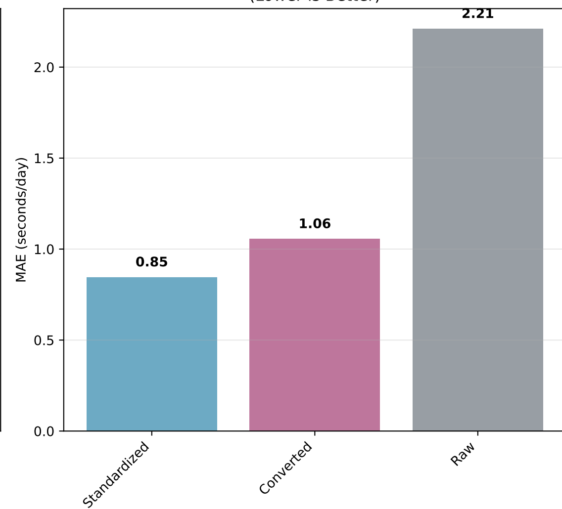
MAE by Time Standardization Method (Lower is Better)
