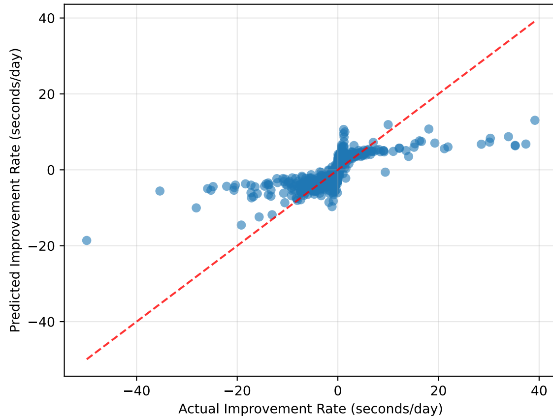
Random Forest R^2 = 0.9145
