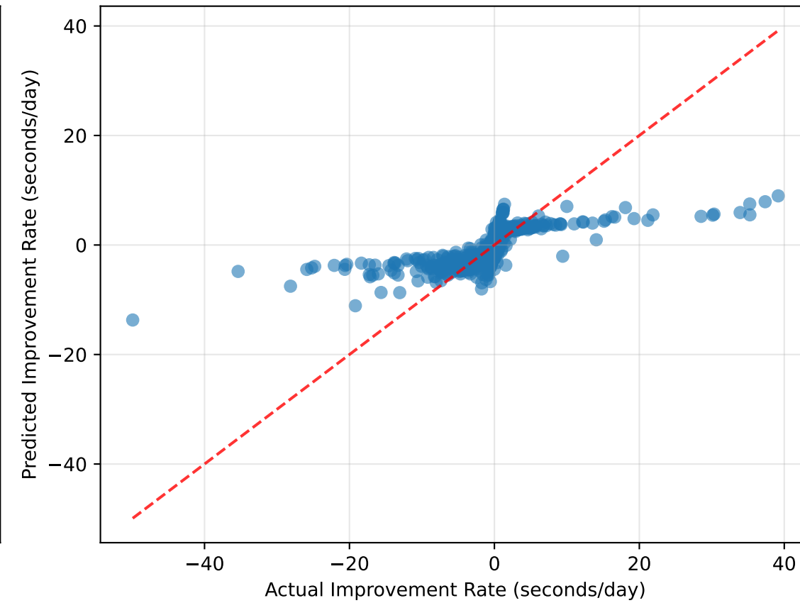
SVR R^2 = 0.5369
