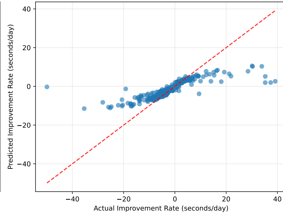
SVR R^2 = 0.5369
