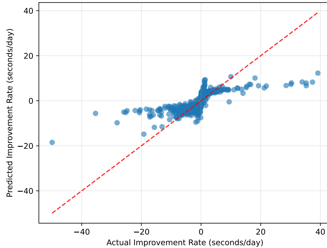
Gradient Boosting R^2 = 0.9021
