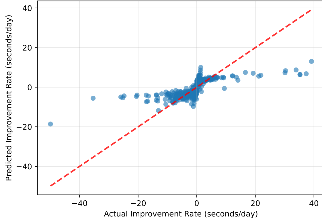
Random Forest R^2 = 0.904 (95% CI: [0.845, 0.954]) n=792
