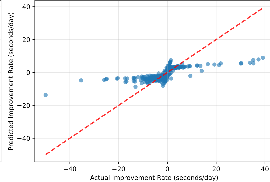
SVR R^2 = 0.505 (95% CI: [0.389, 0.659]) n=792
