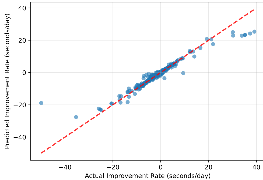
Random Forest R^2 = 0.904 (95% CI: [0.845, 0.954]) n=792
