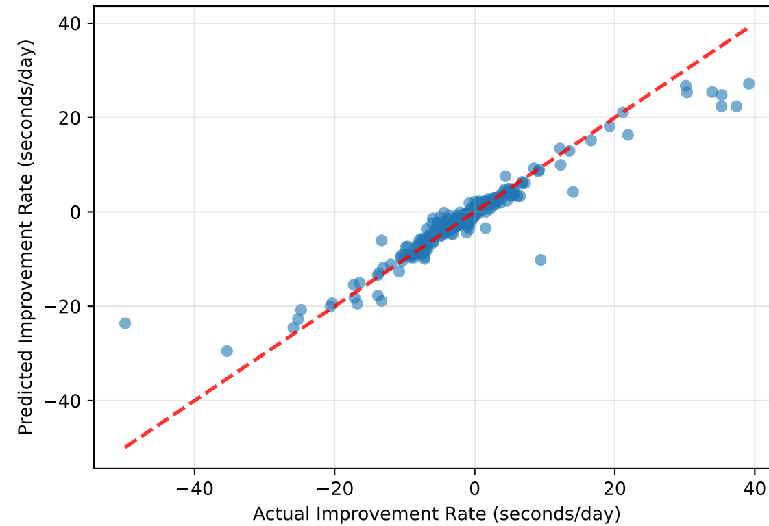
Gradient Boosting R^2 = 0.894 (95% CI: [0.840, 0.936]) n=792
