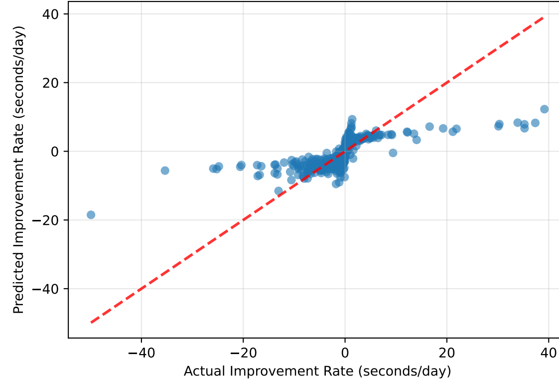
Gradient Boosting R^2 = 0.894 (95% CI: [0.840, 0.936]) n=792
