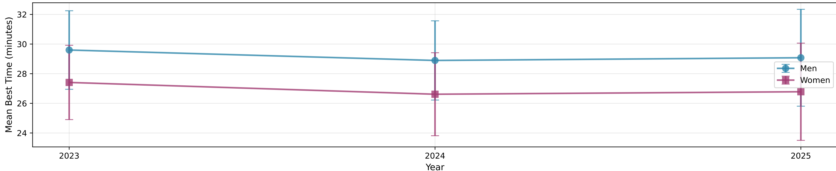
Summary Statistics
