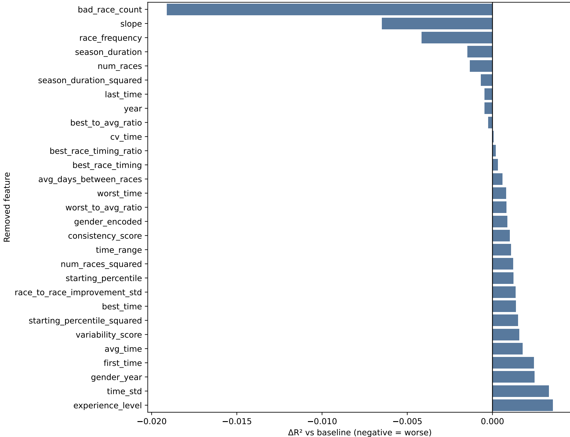
Feature ablation: \Delta R^2 after removing one feature (Train 2023 \rightarrow Test 2024, Random Forest)
