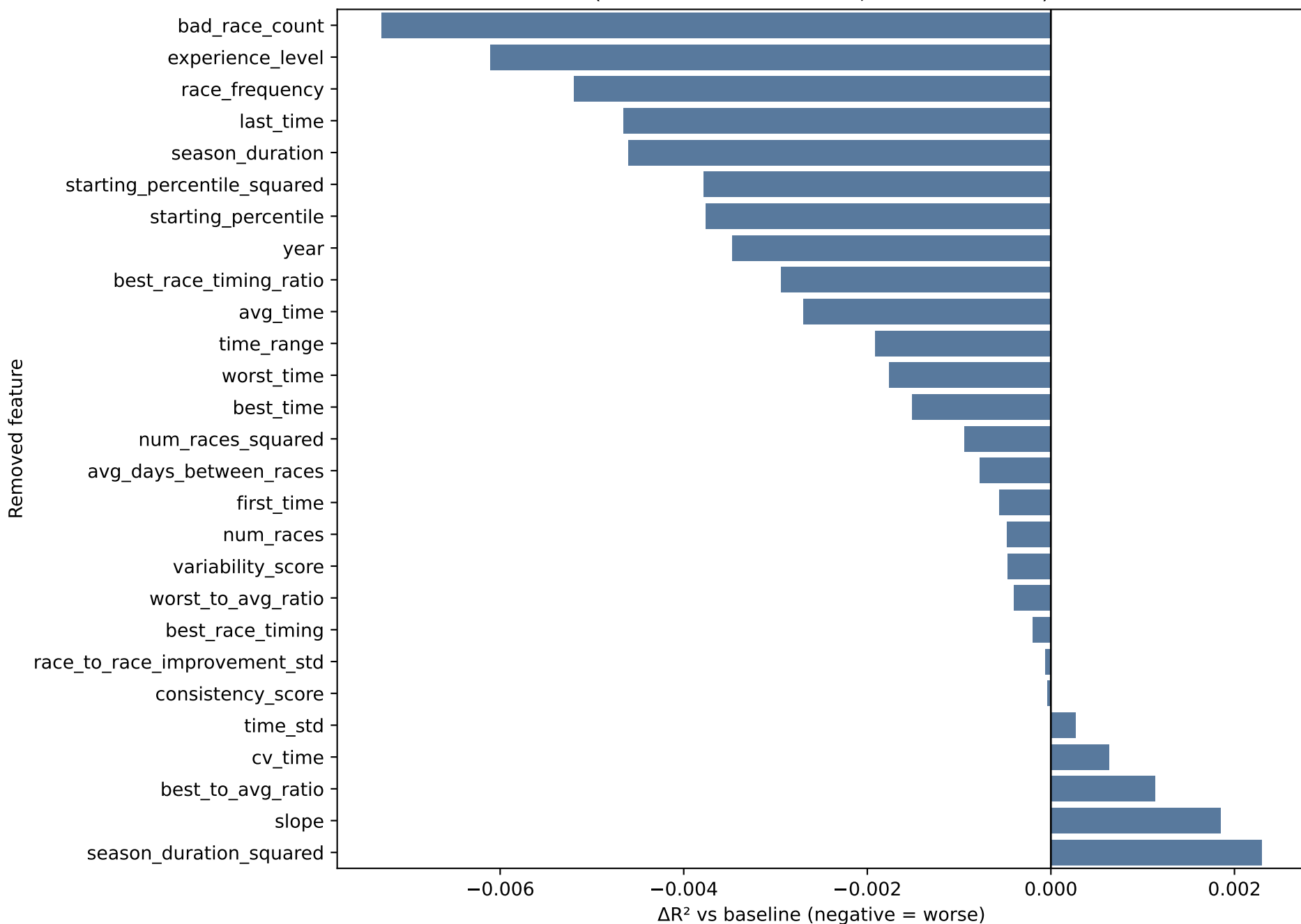
Feature ablation: \Delta R^2 after removing one feature (F only) (Train 2023 \rightarrow Test 2024, Random Forest)
