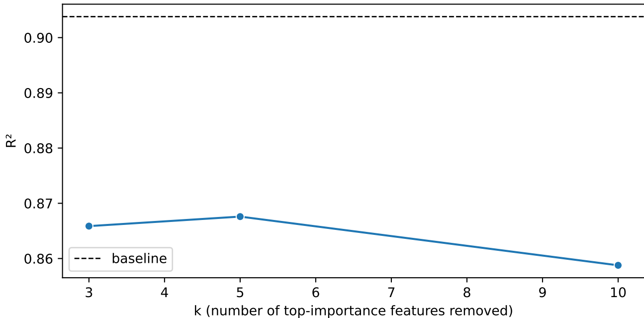
Drop top-k important features: R^2 (Train 2023 \rightarrow Test 2024, Random Forest)
