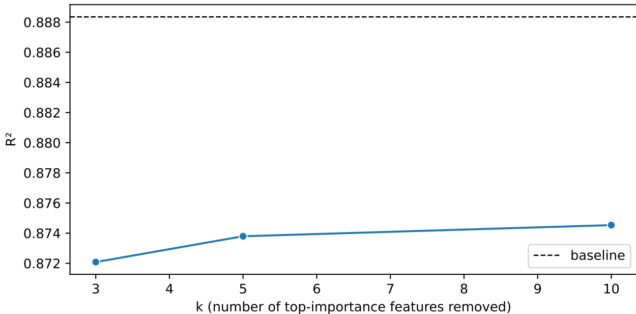
Drop top-k important features: R^2 (F only) (Train 2023 \rightarrow Test 2024, Random Forest)
