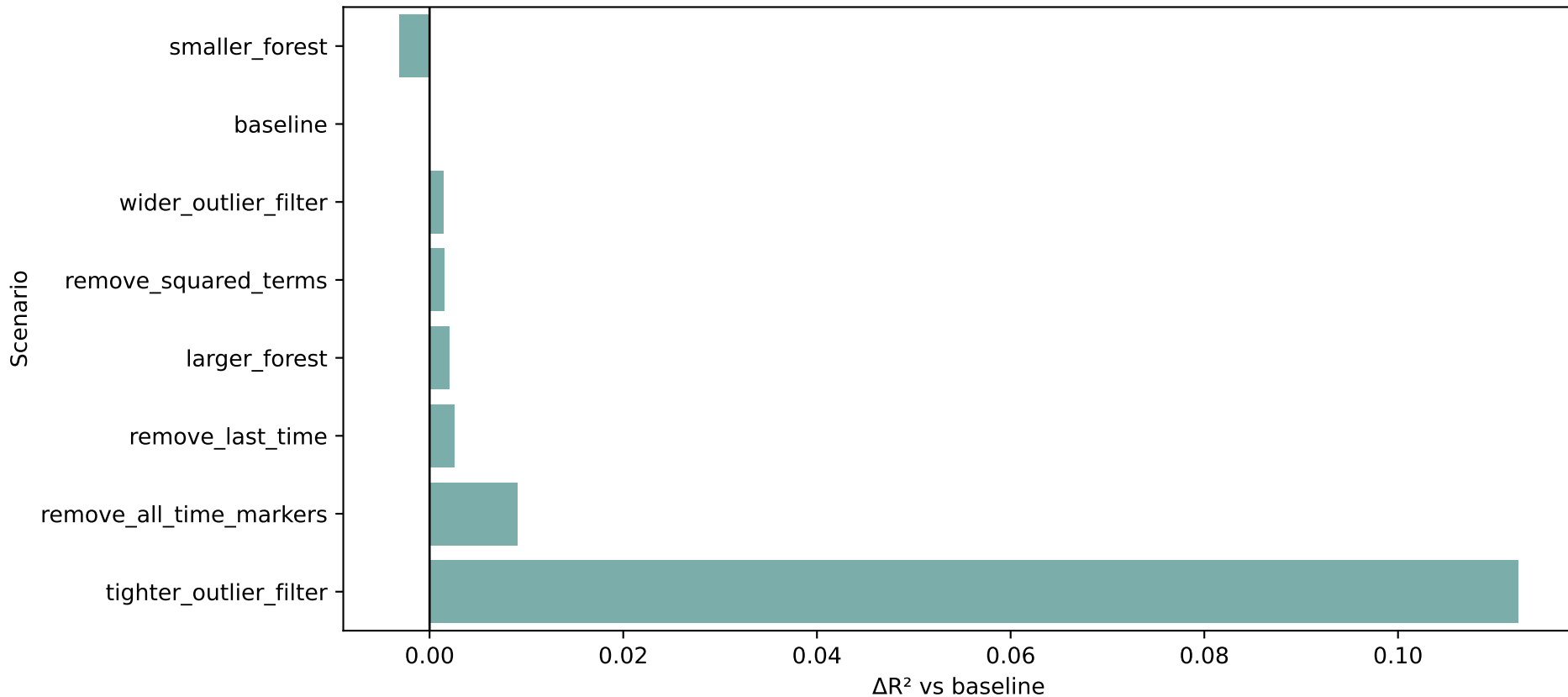
Sensitivity sweep: \Delta R^2 vs baseline (M only) (Train 2023 \rightarrow Test 2024, Random Forest)
