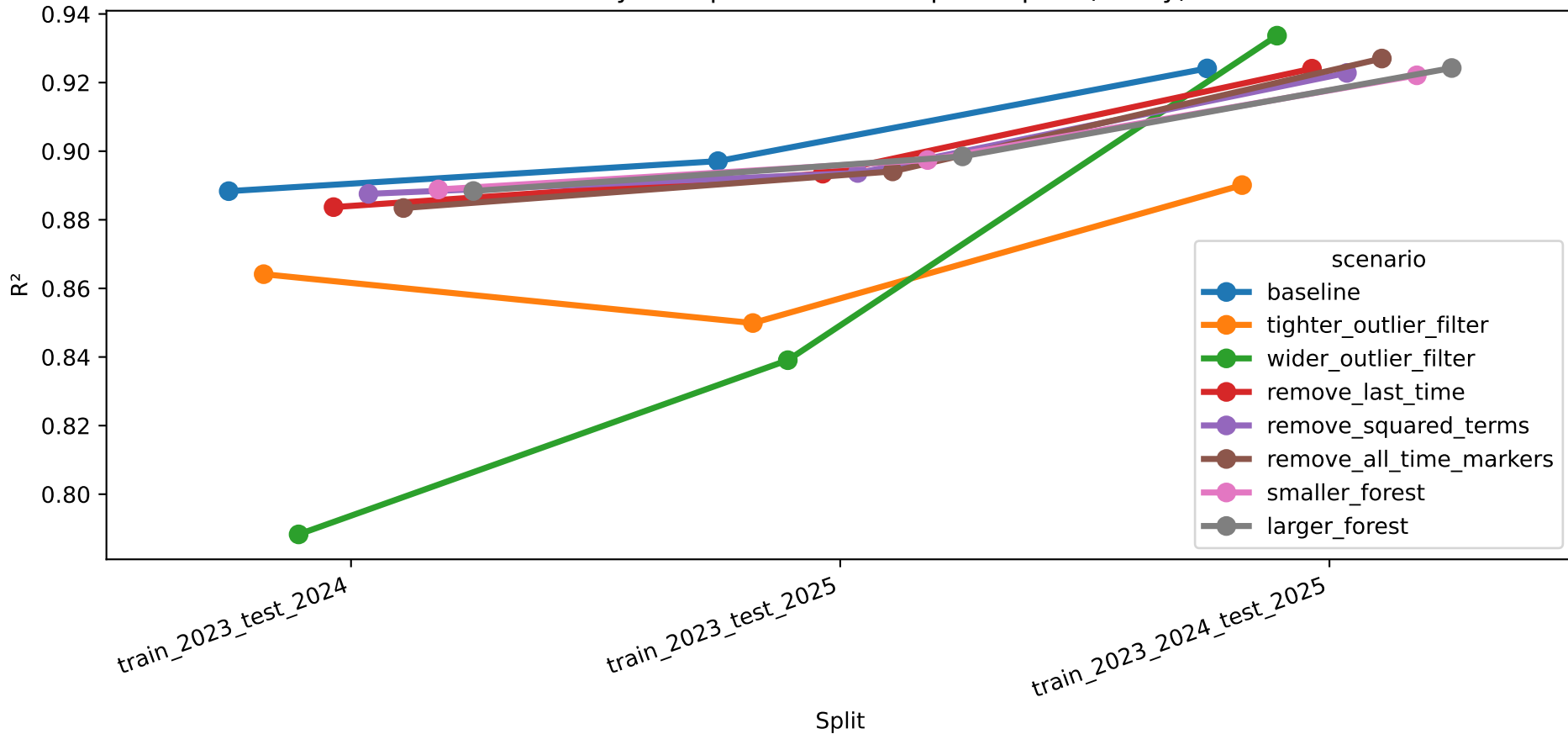
Sensitivity sweep: R^2 across temporal splits (F only)
