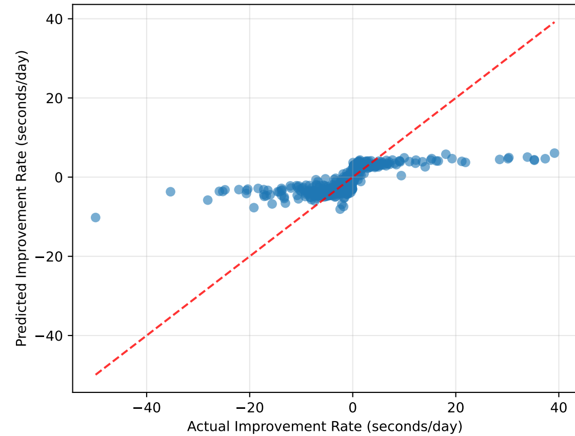
SVR R^2 = 0.4486
