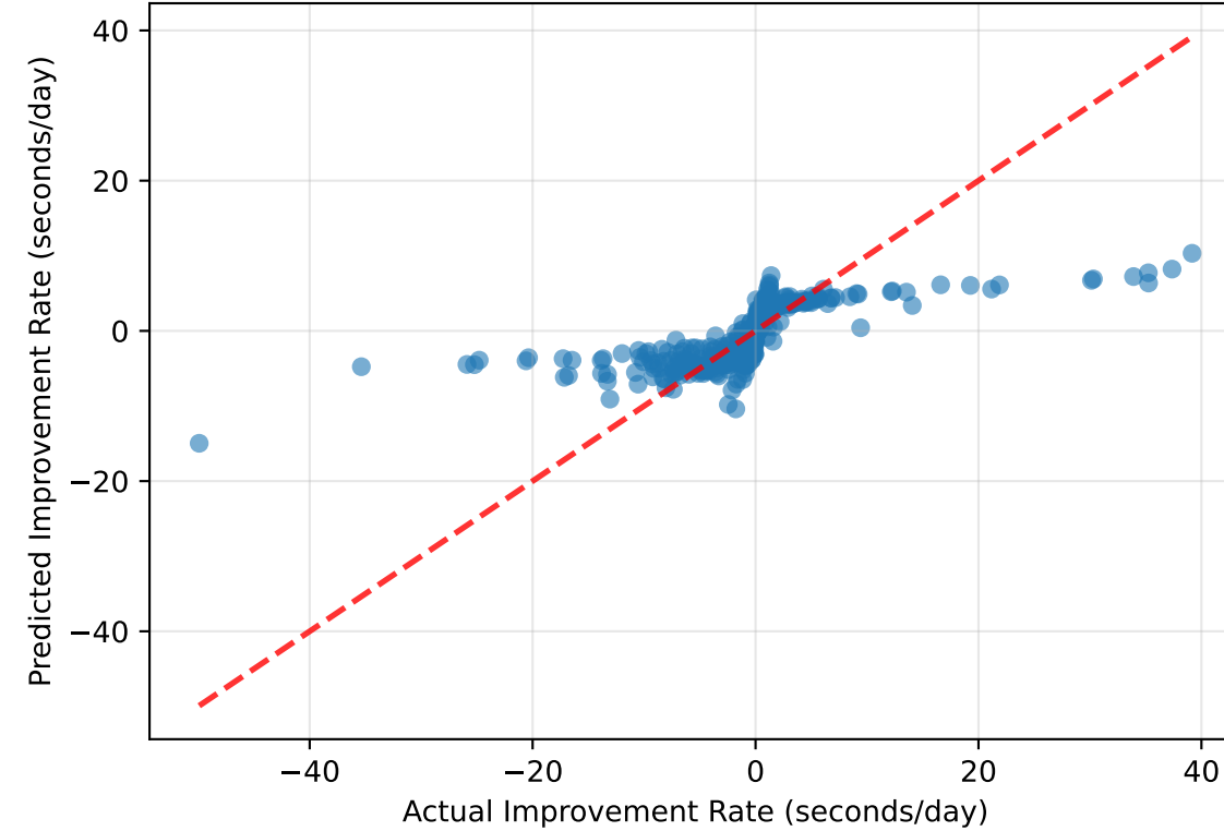
Gradient Boosting R^2 = 0.895 (95% CI: [0.831, 0.947]) n=792
