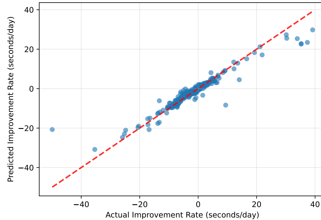
Gradient Boosting R^2 = 0.895 (95% CI: [0.831, 0.947]) n=792
