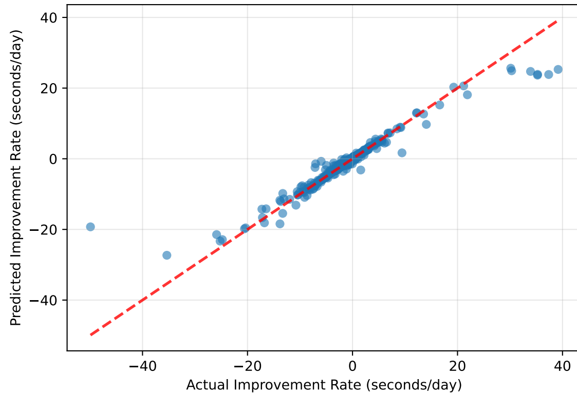
Random Forest R^2 = 0.910 (95% CI: [0.846, 0.956]) n=792
