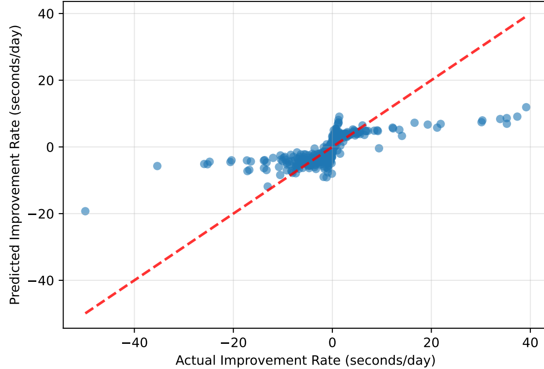
Random Forest R^2 = 0.910 (95% CI: [0.846, 0.956]) n=792
