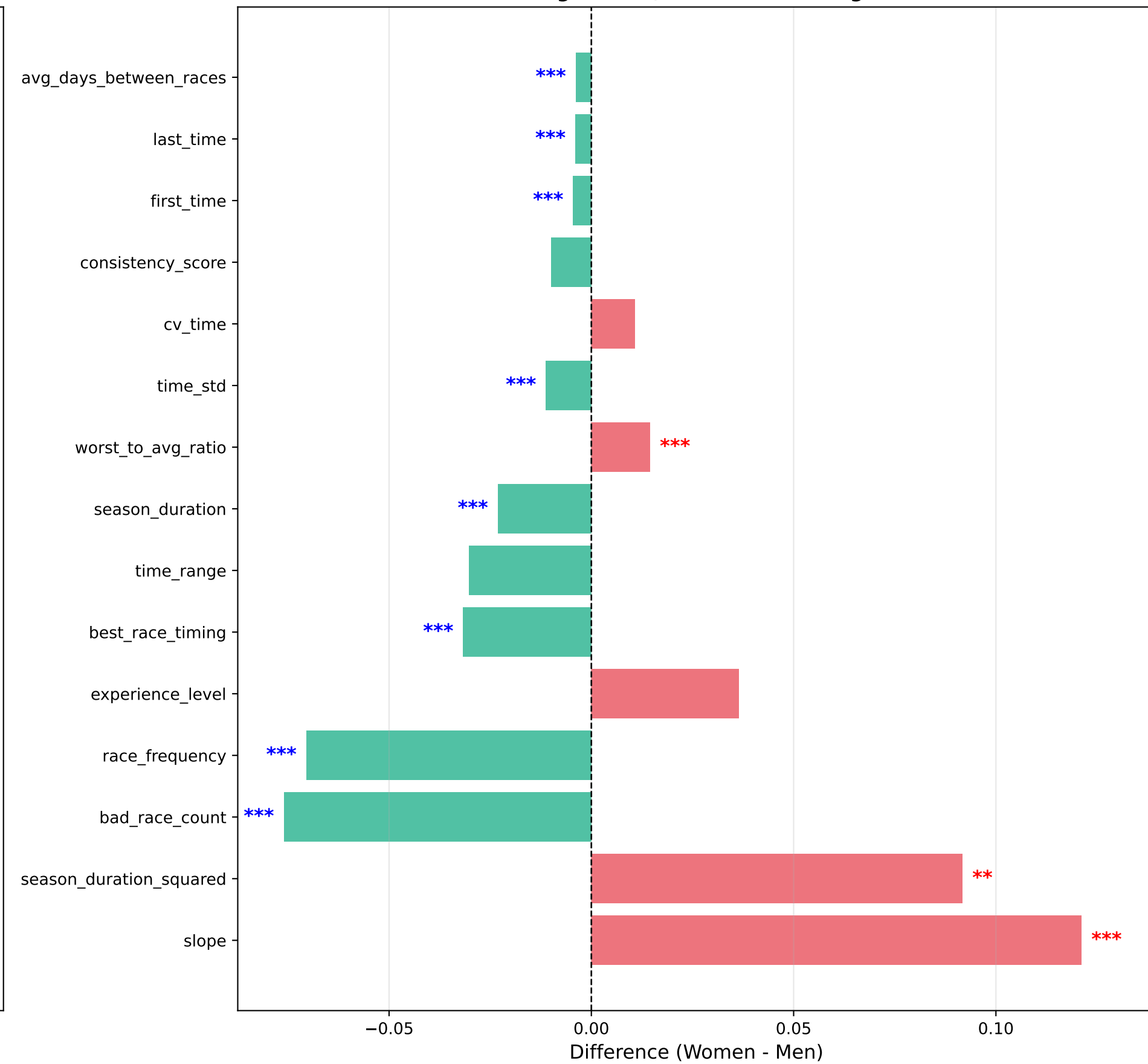
Feature Importance Differences (Red/Green = FDR Significant, Gray = Not Significant) FDR: 15 significant, Bonferroni: 10 significant
