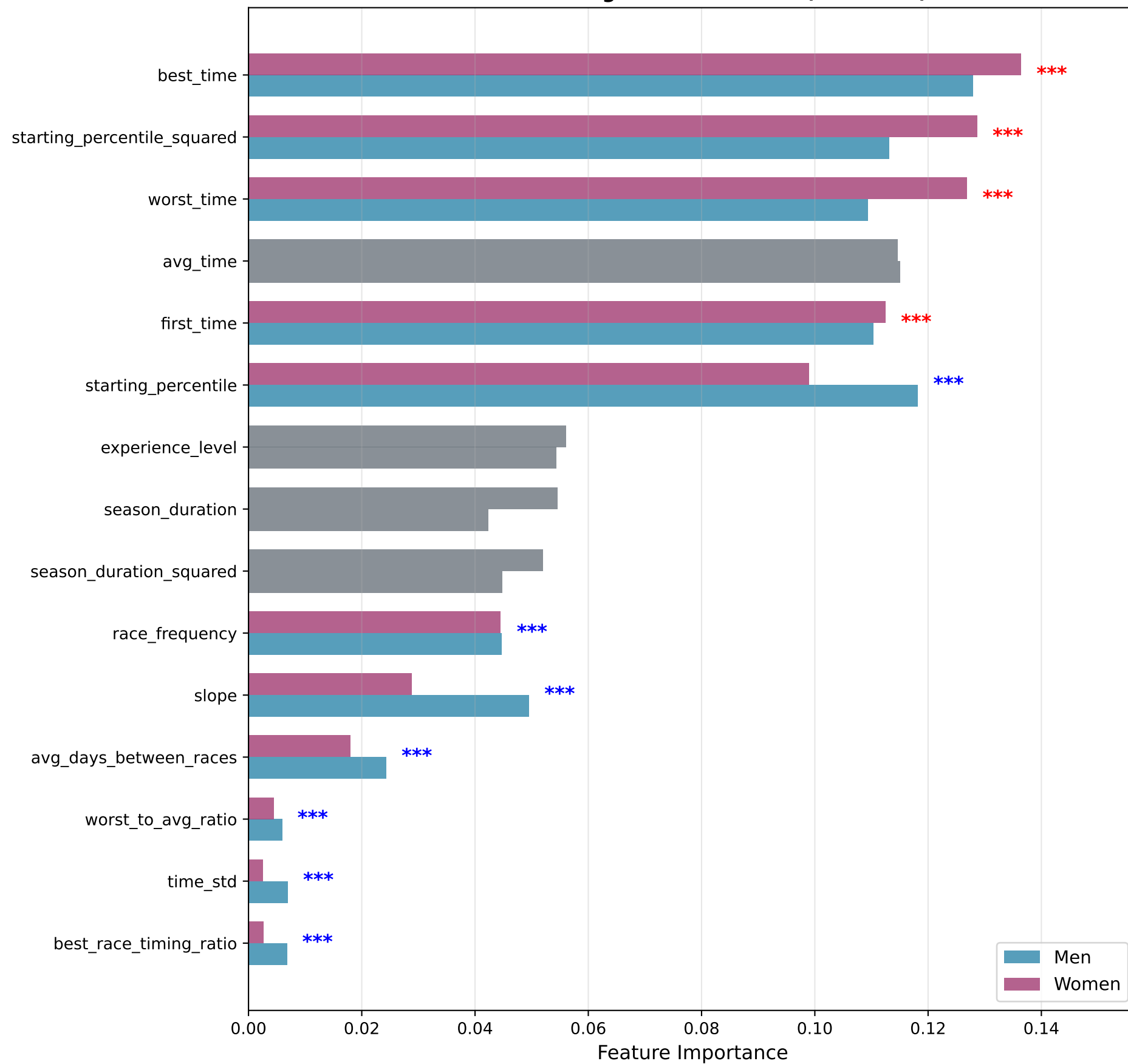
Random Forest Feature Importance Comparison: Men vs Women (Colored = Bonferroni Significant Between Genders, ***p<Bonferroni threshold) Bonferroni Significant: 16 total (11 shown)
