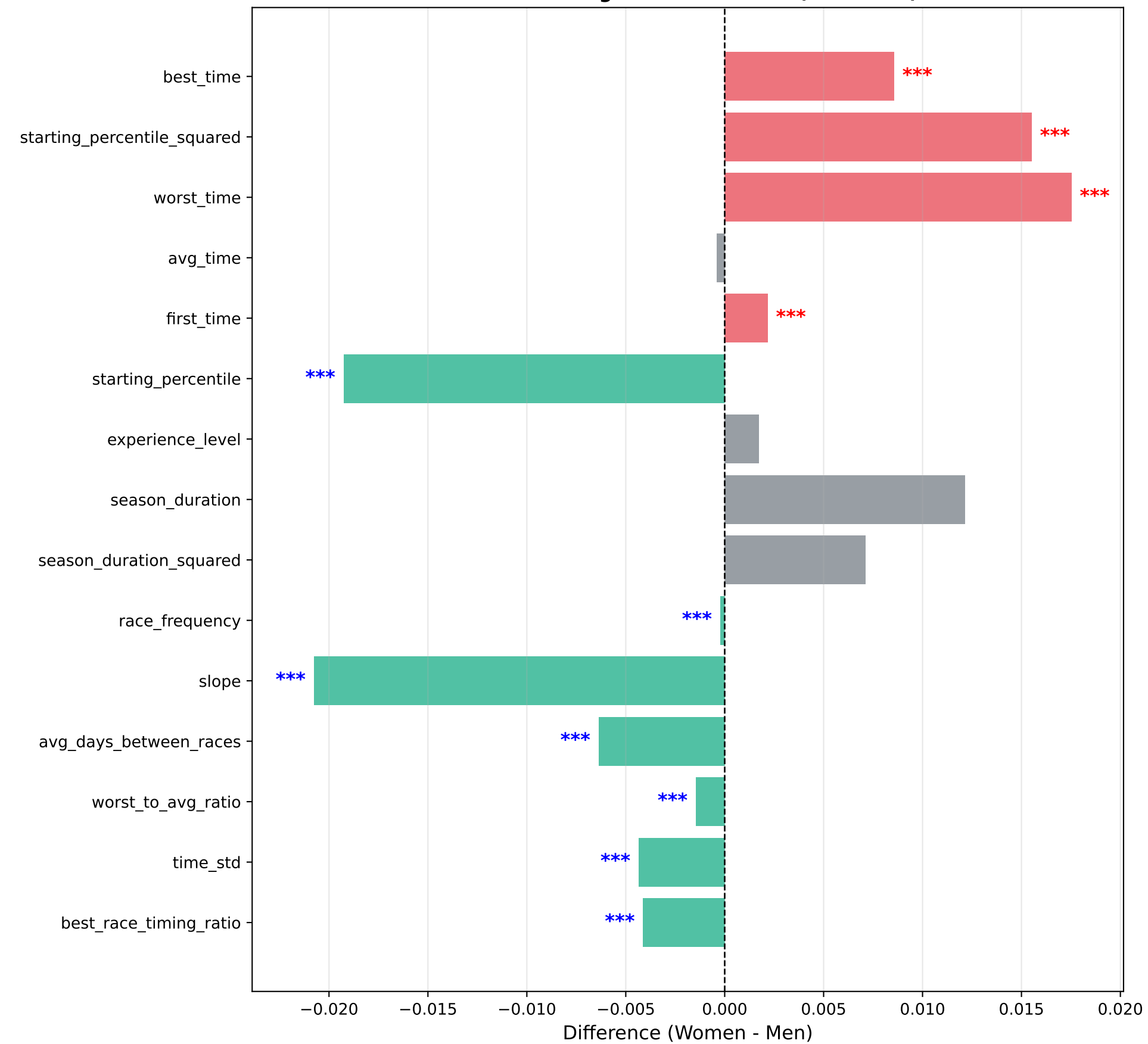
Random Forest Feature Importance Differences (Red/Green = Bonferroni Significant Between Genders, Gray = Not Significant) Bonferroni Significant: 16 total (11 shown)
