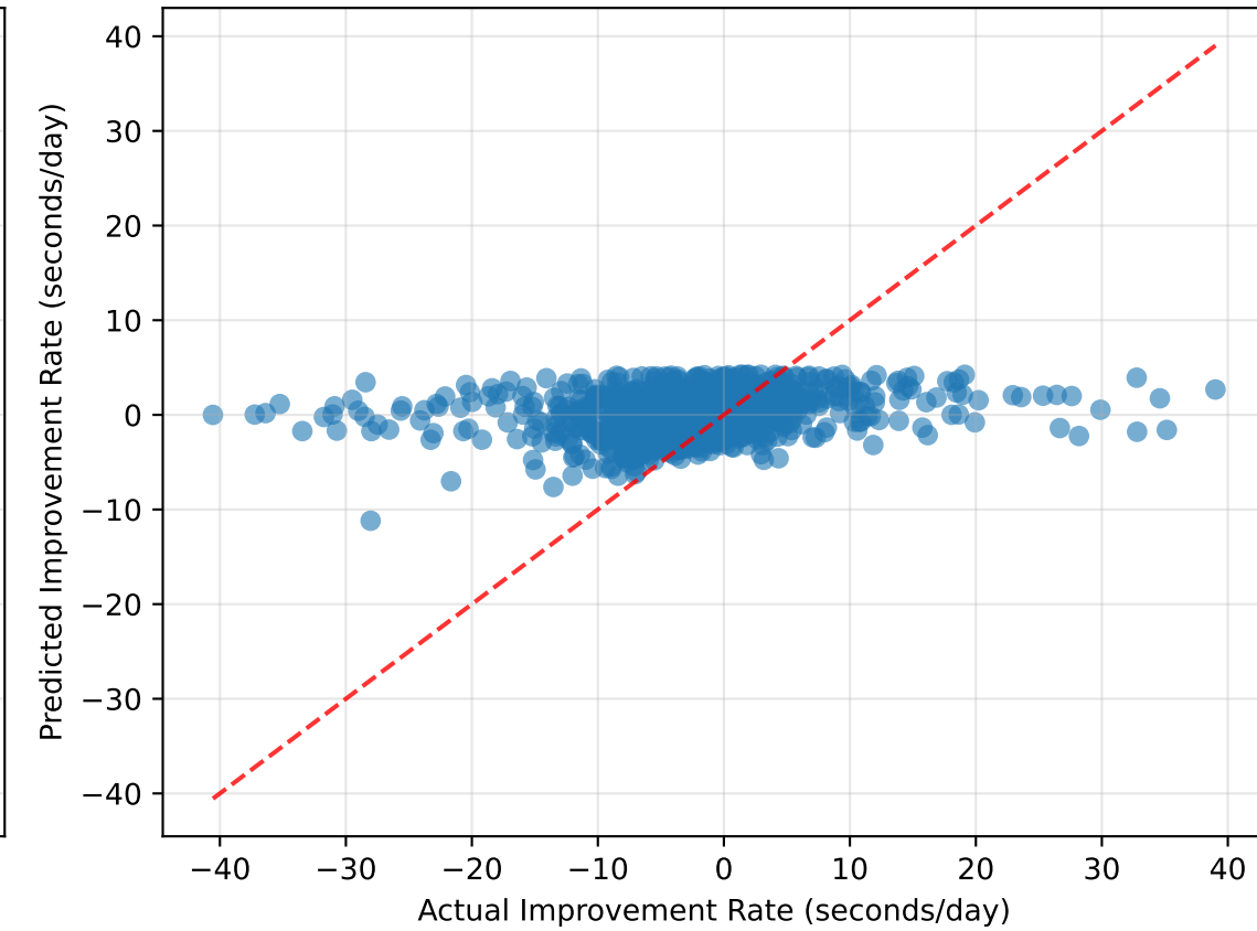
SVR R^2 = 0.0407
