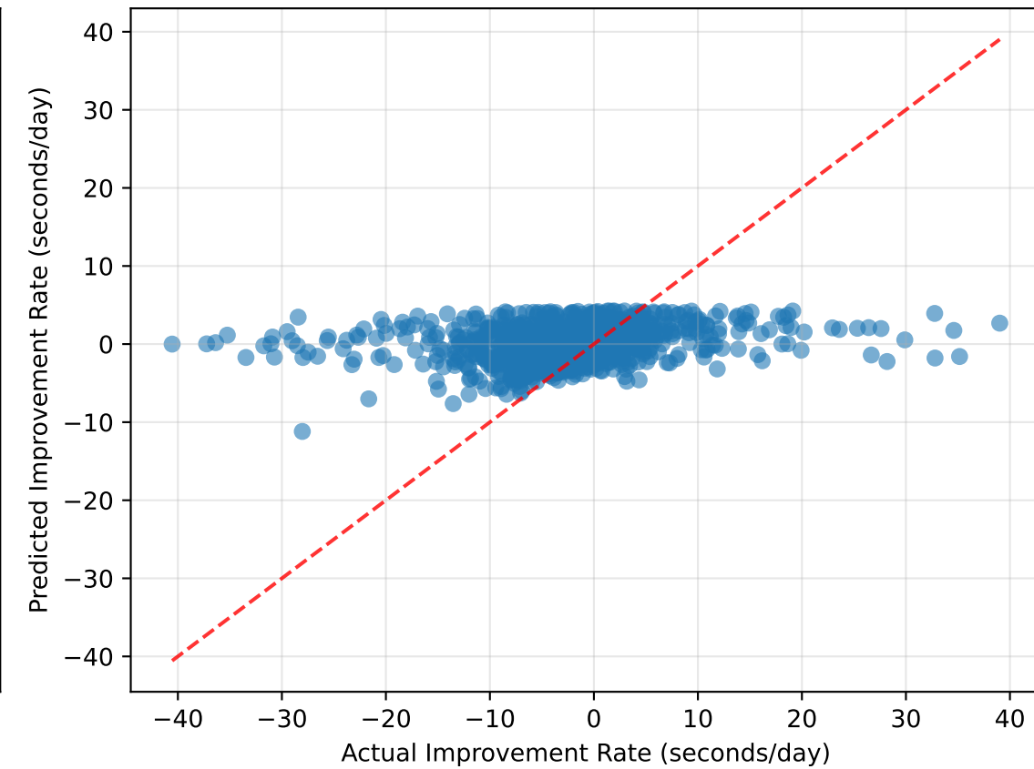
SVR R^2 = 0.0407
