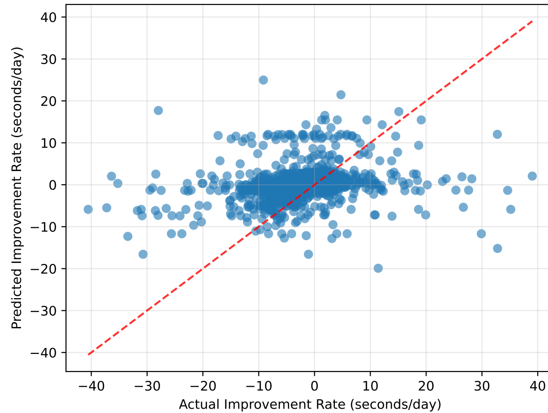
Gradient Boosting R^2 = -0.1289
