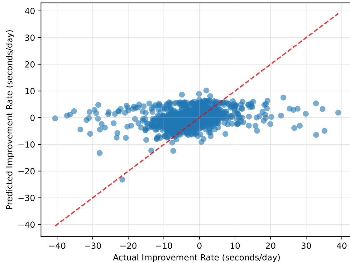
Random Forest R^2 = -0.3317
