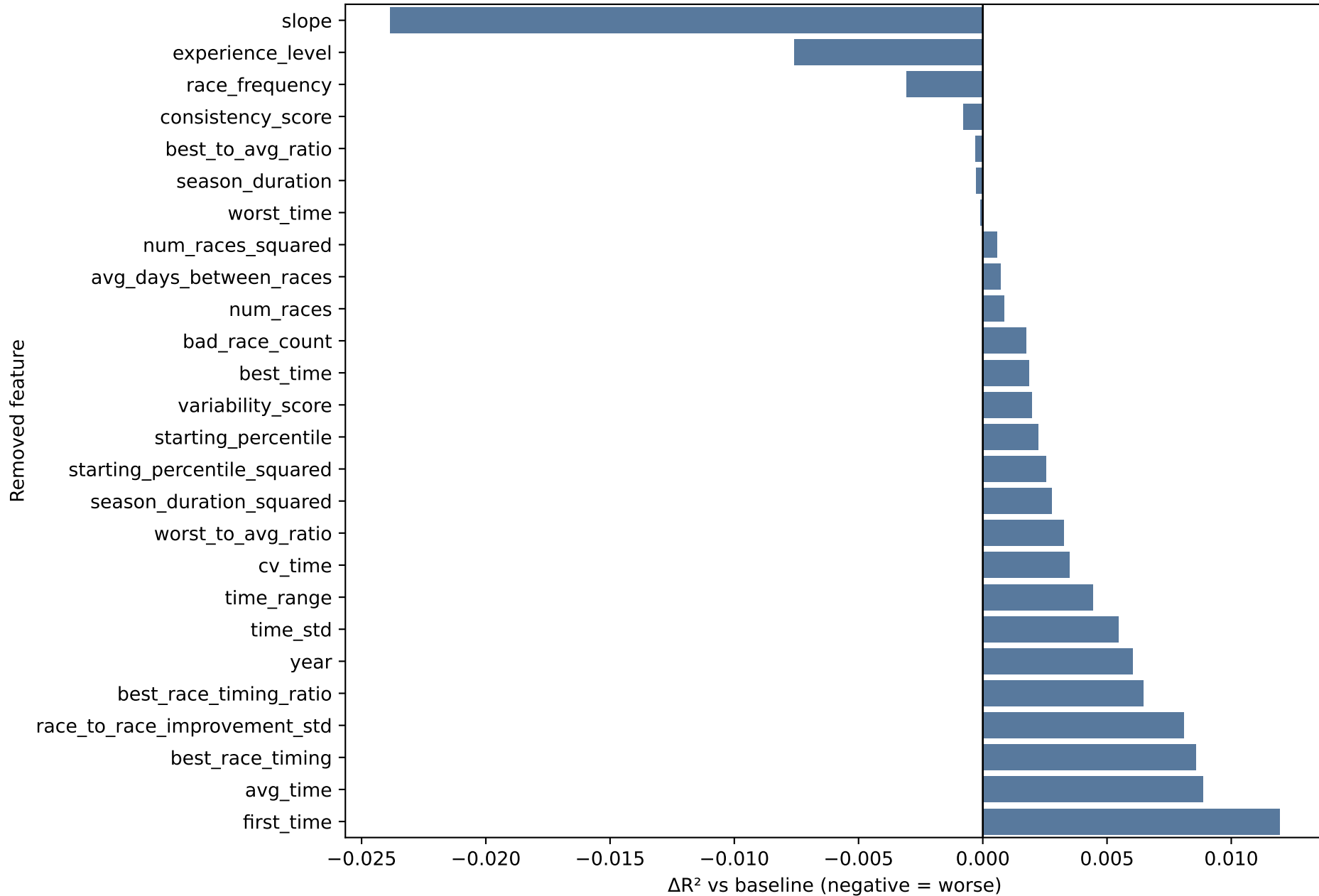
Feature ablation: \Delta R^2 after removing one feature (M only) (Train 2023 \rightarrow Test 2024, Random Forest)
