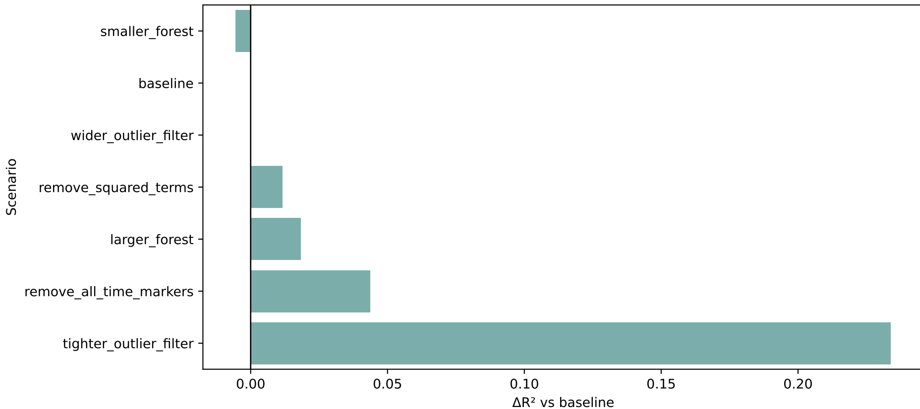
Sensitivity sweep: \Delta R^2 vs baseline (F only) (Train 2023 \rightarrow Test 2024, Random Forest)
