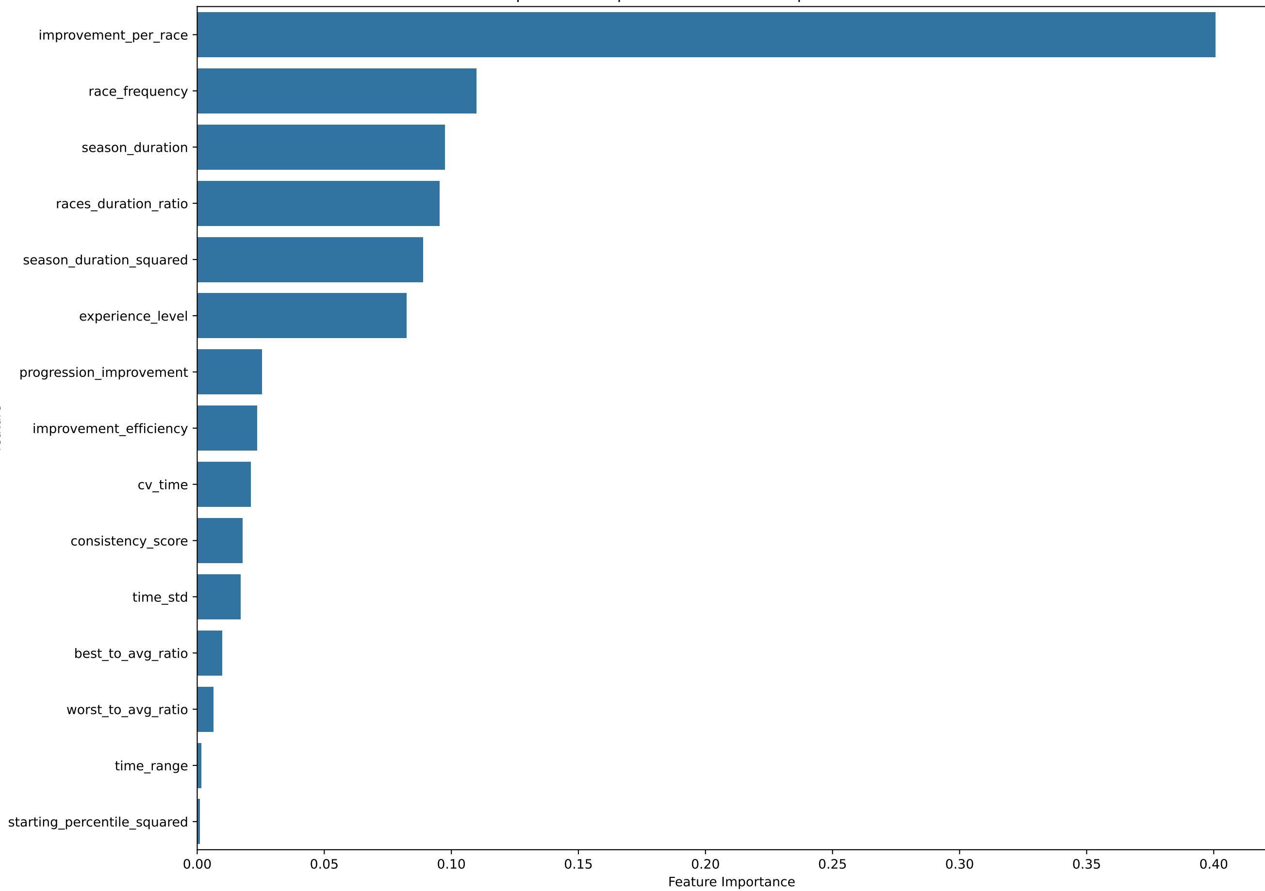
Top 15 Most Important Features for Improvement Prediction
