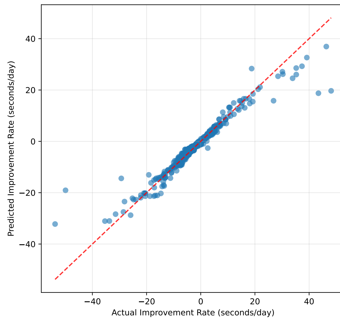
Gradient Boosting R^2 = 0.9195
