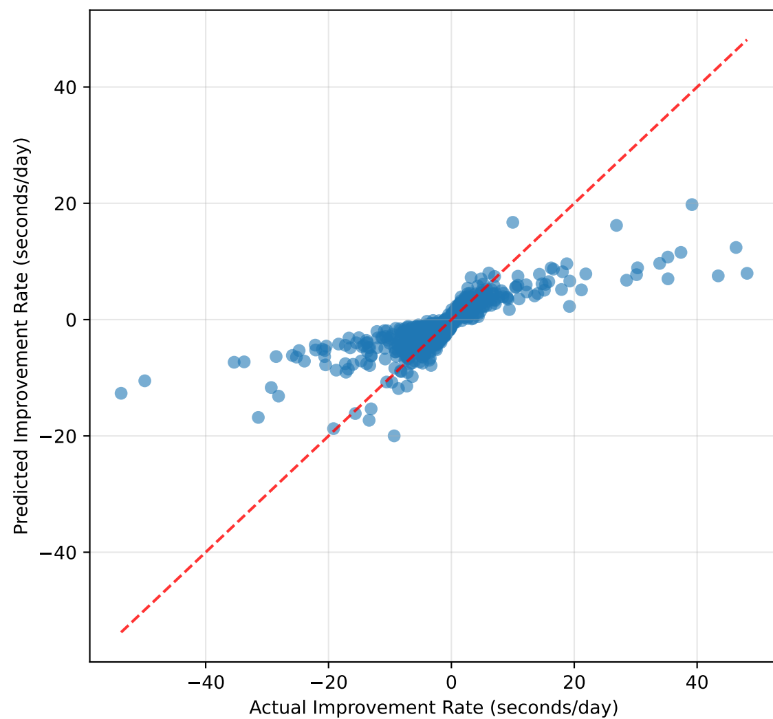
Random Forest R^2 = 0.9115
