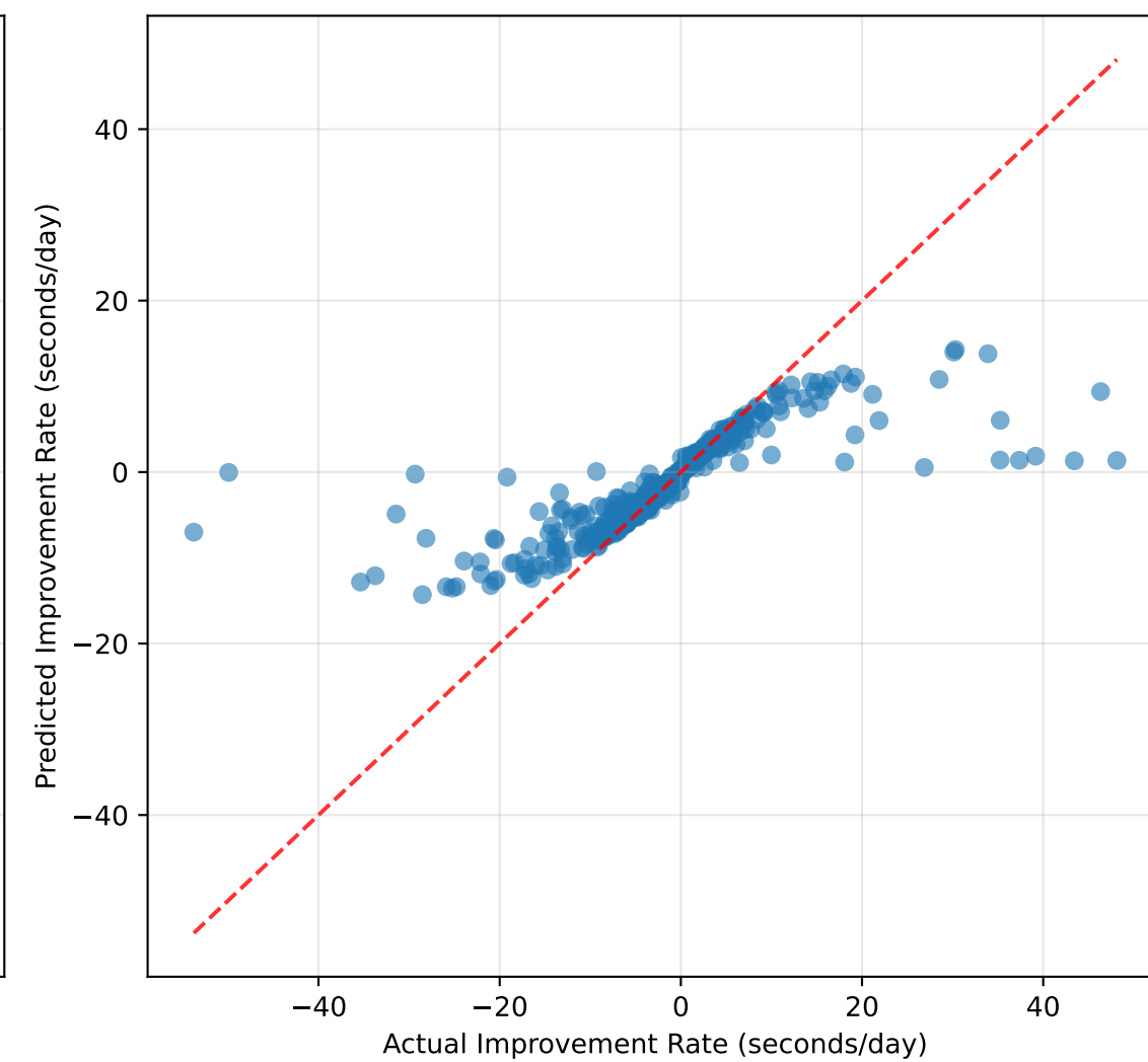
SVR R^2 = 0.5568
