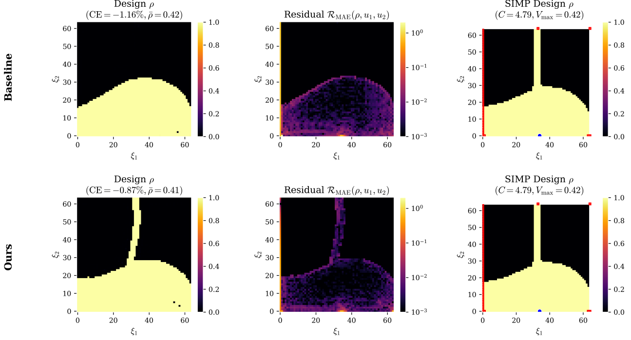
Figure 3. Mechanics topology optimization (Baseline vs. REPA-P). Each row shows (left→right) the generated density \rho with CE (%) and mean \bar{\rho} , the equilibrium residual \mathcal{R}_{\text{MAE}}(\rho, u_1, u_2) (log scale; lower is better), and the SIMP reference with compliance C and volume limit V_{\text{max}} (red: displacement BCs; blue: load). REPA-P yields cleaner slender members and lower residuals than the baseline under the same volume constraint.
