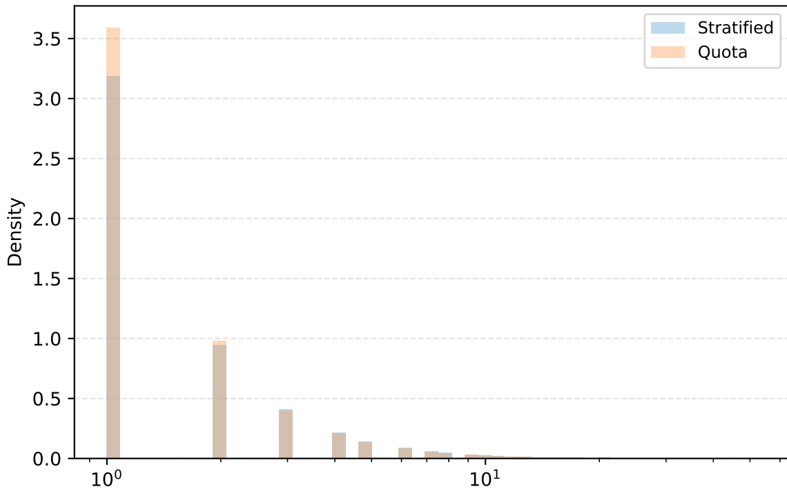
issues\_closed
