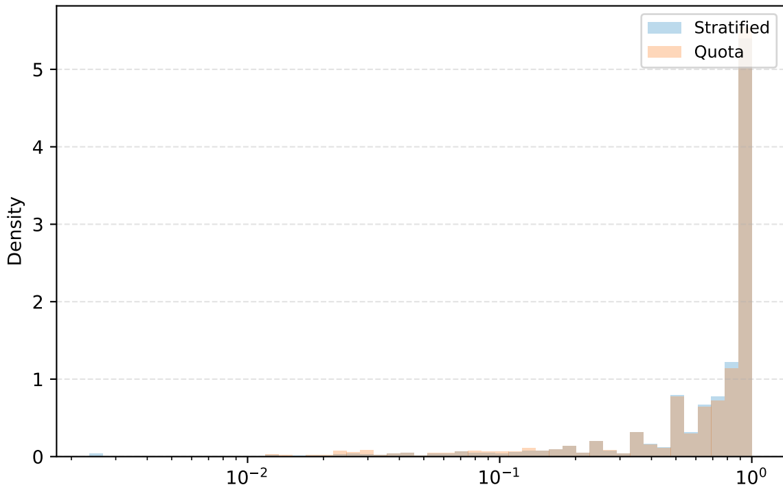
pr_merge_ratio
