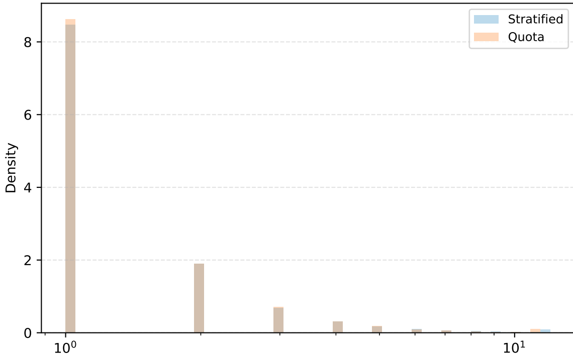
bug\_issues\_external
