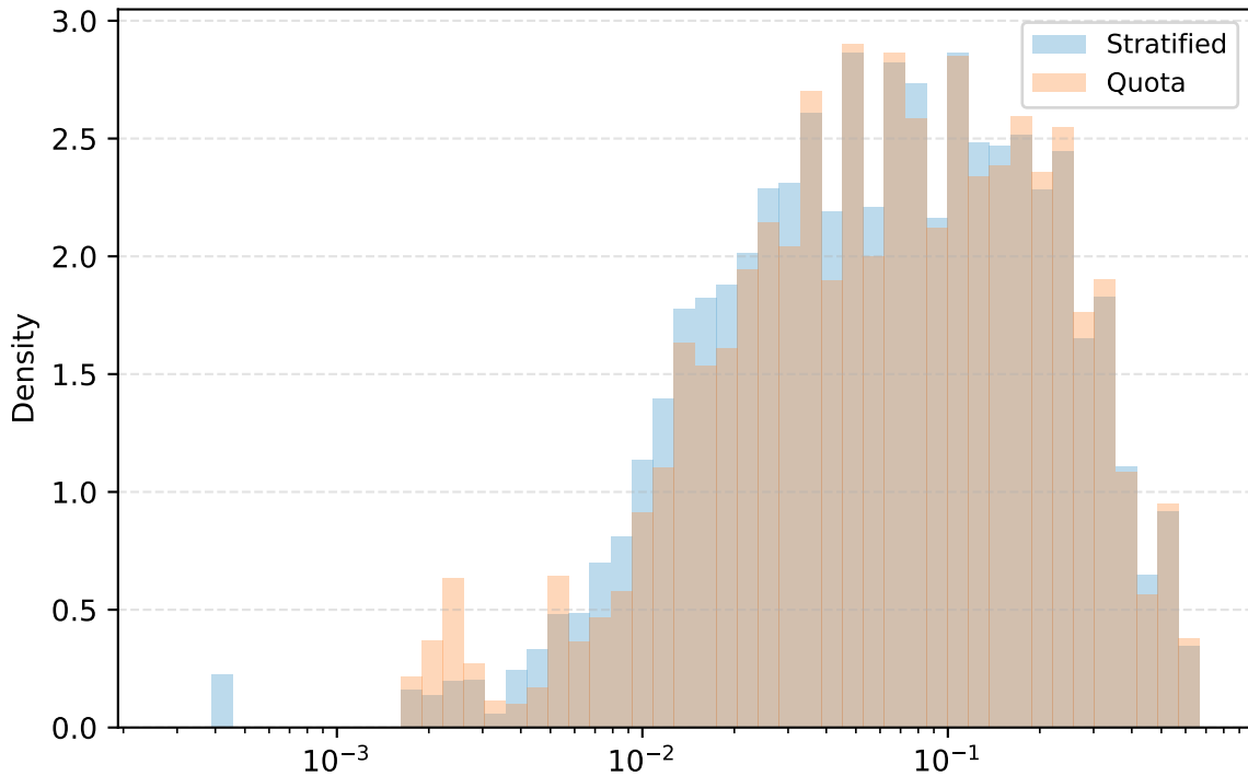
merge\_ratio
