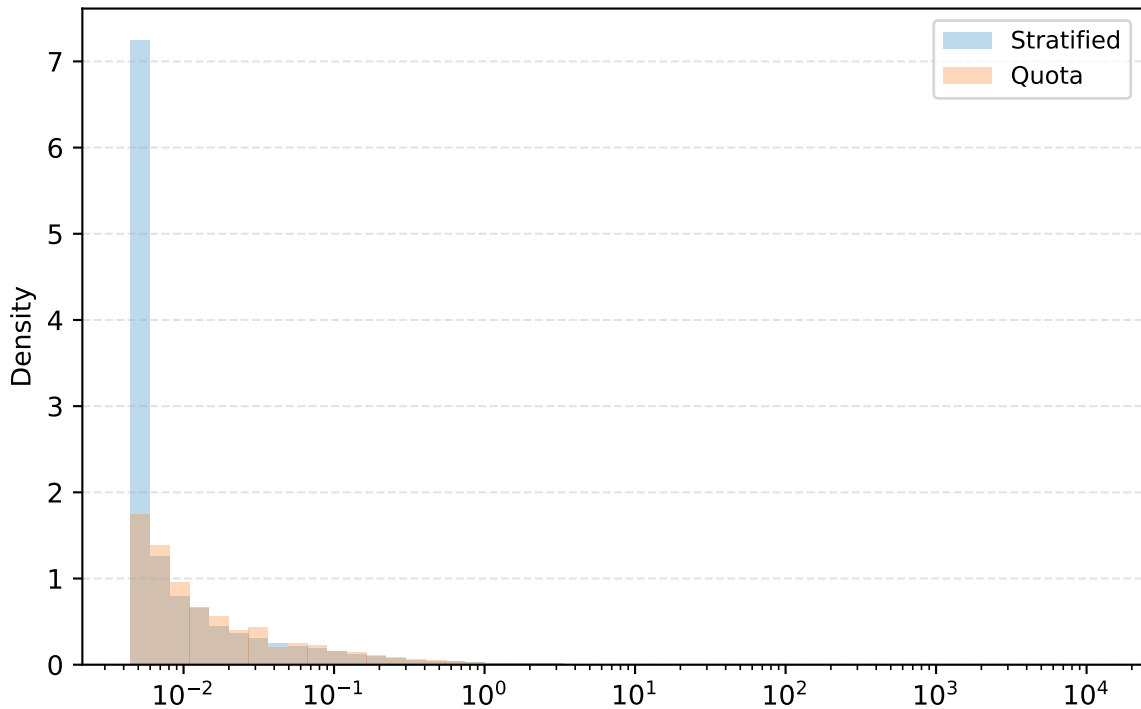
pr\_latency\_hours\_avg
