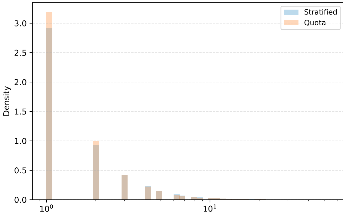
issues\_opened
