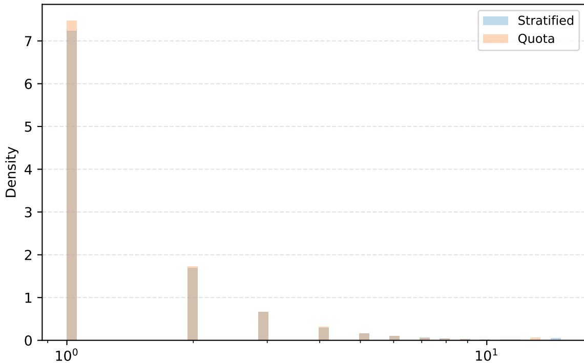
bug\issues
