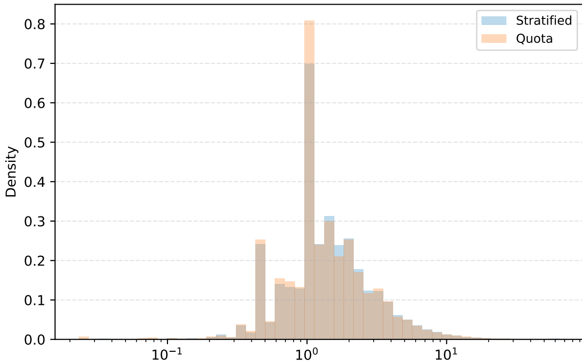
files\_changed\_per\_commit
