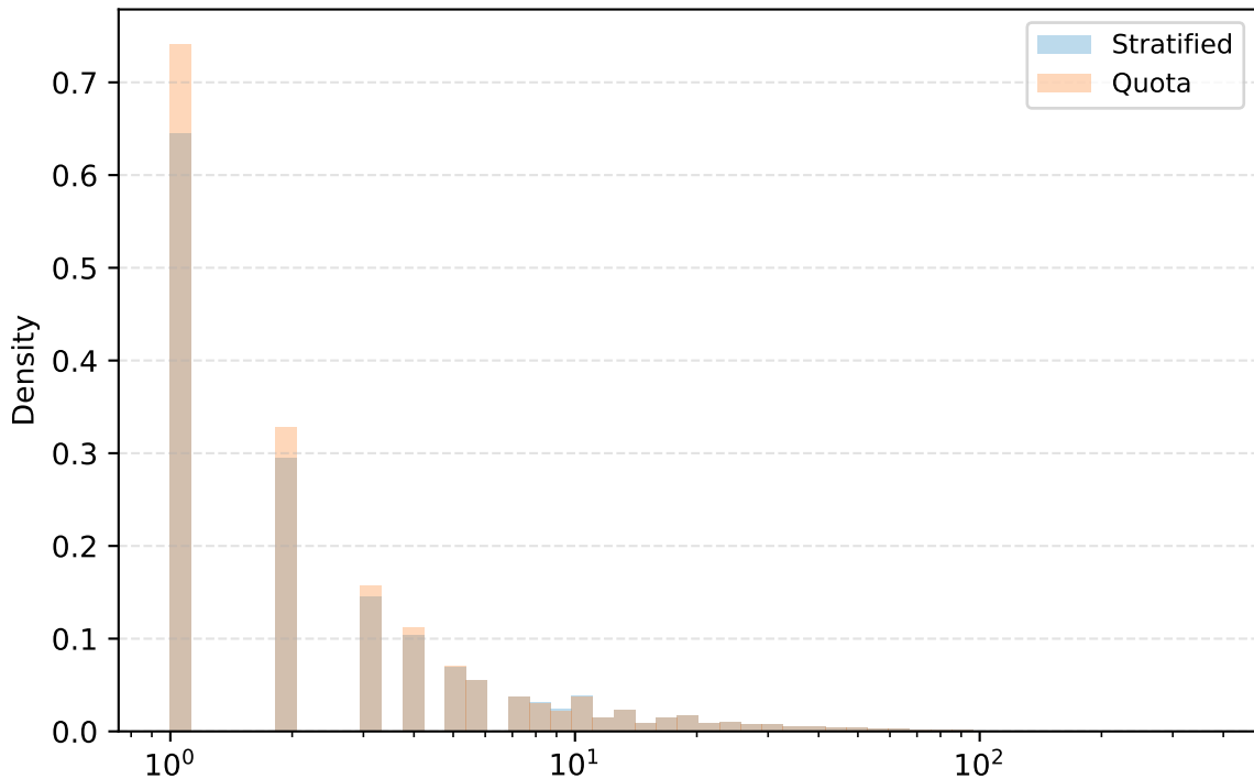
commits\_per\_month
