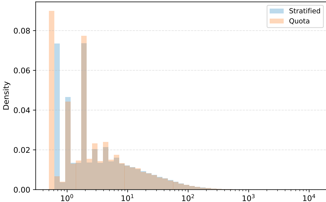
avg\_churn\_per\_commit
