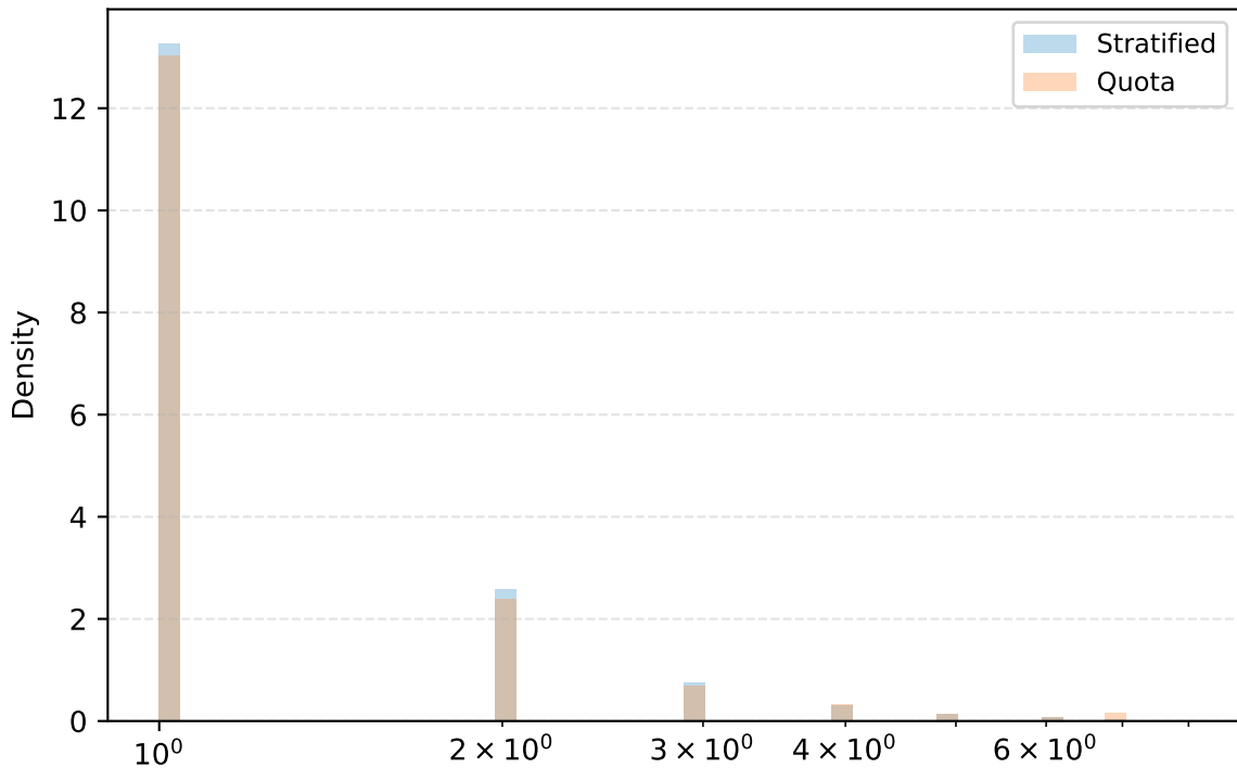
releases\_per\_month
