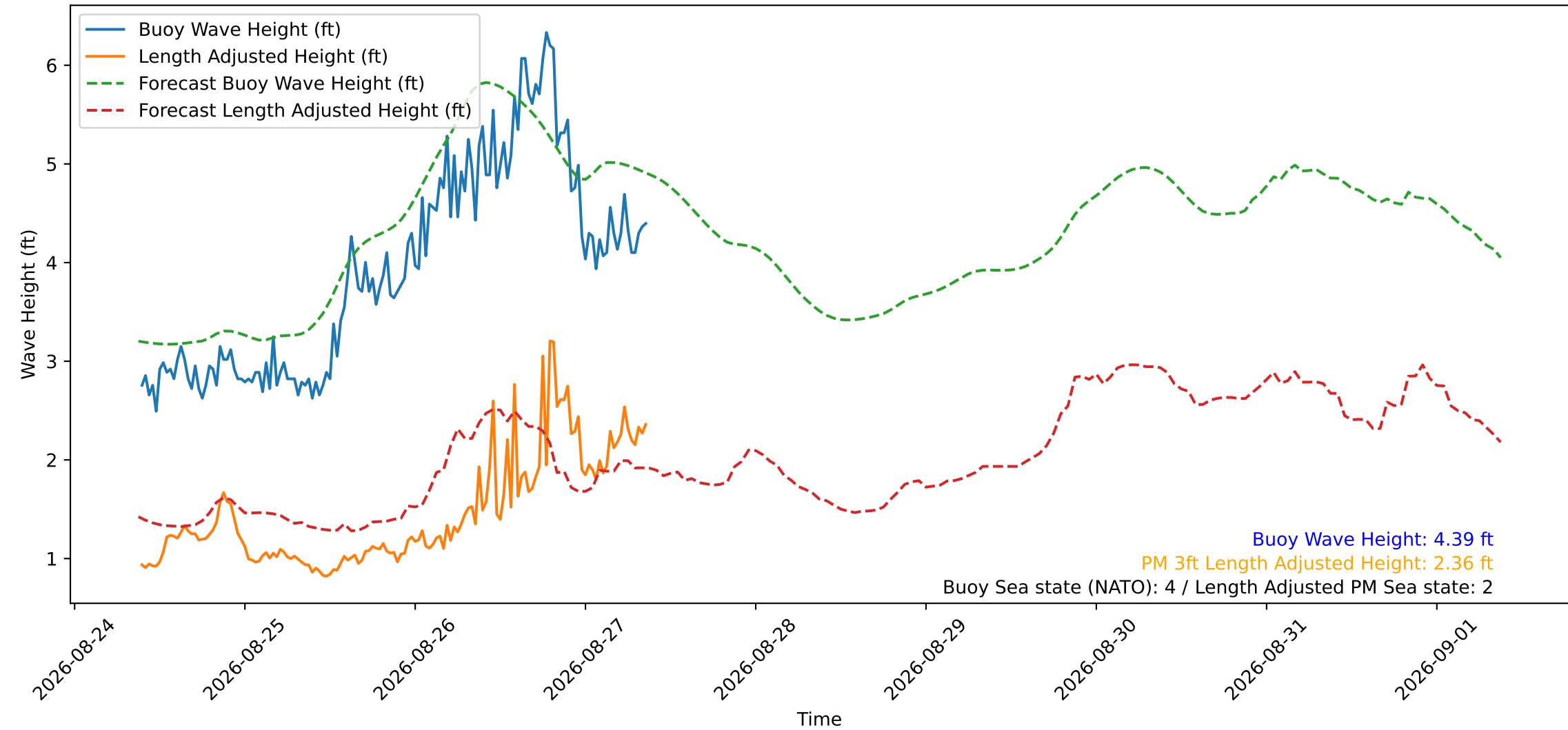
Wave Heights over Time for Green Beach at 2026-08-27 09:21:16
