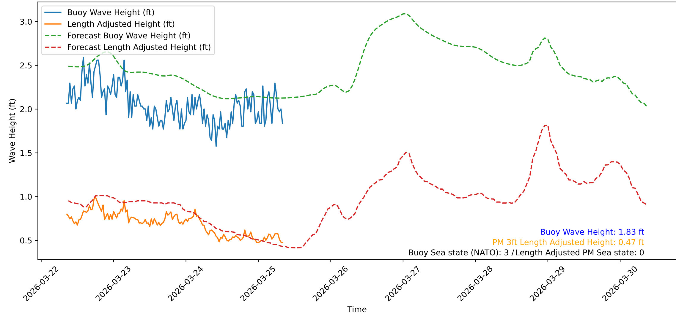
Wave Heights over Time for Oceanside Harbor at 2026-03-25 08:30:31
