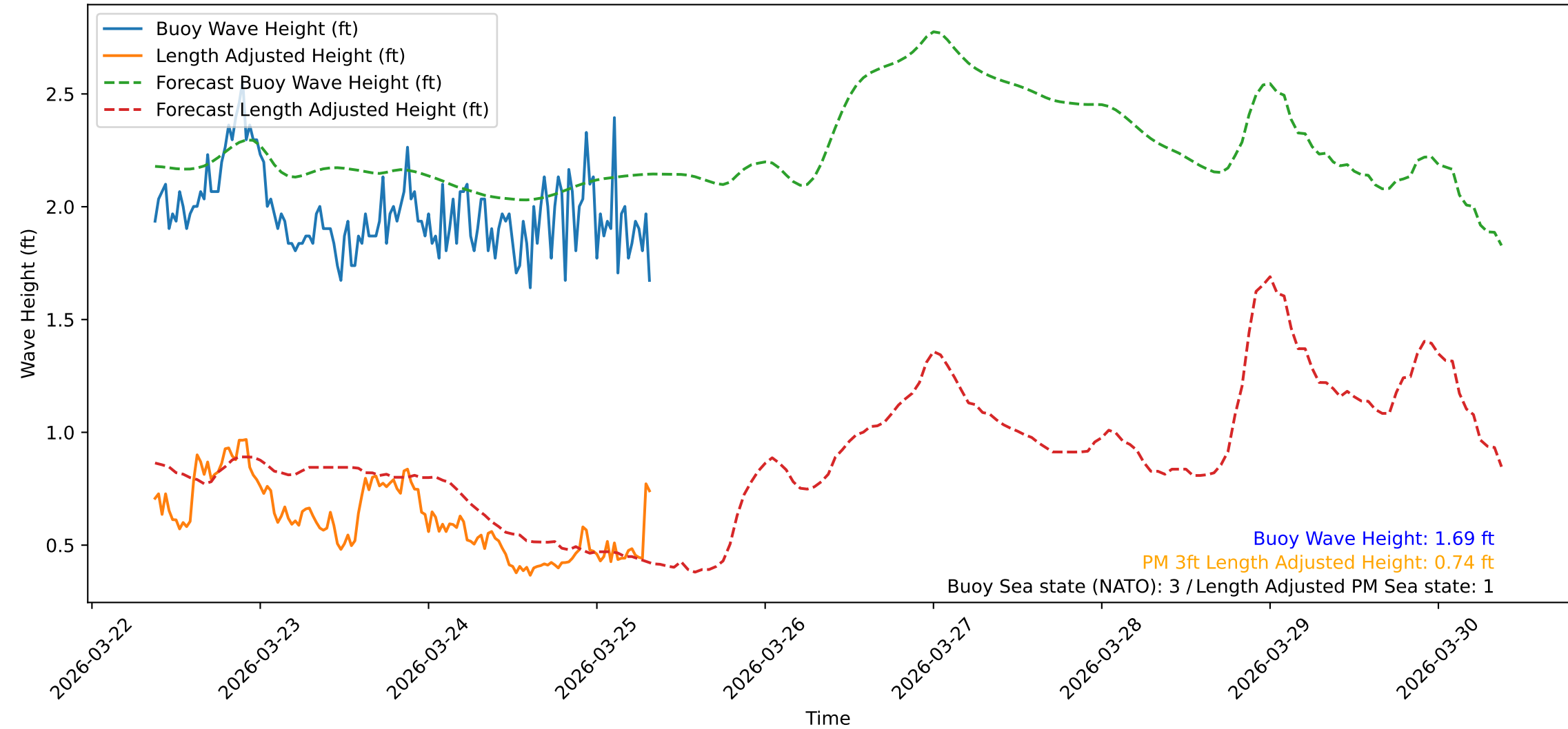
Wave Heights over Time for Red Beach at 2026-03-25 08:30:48
