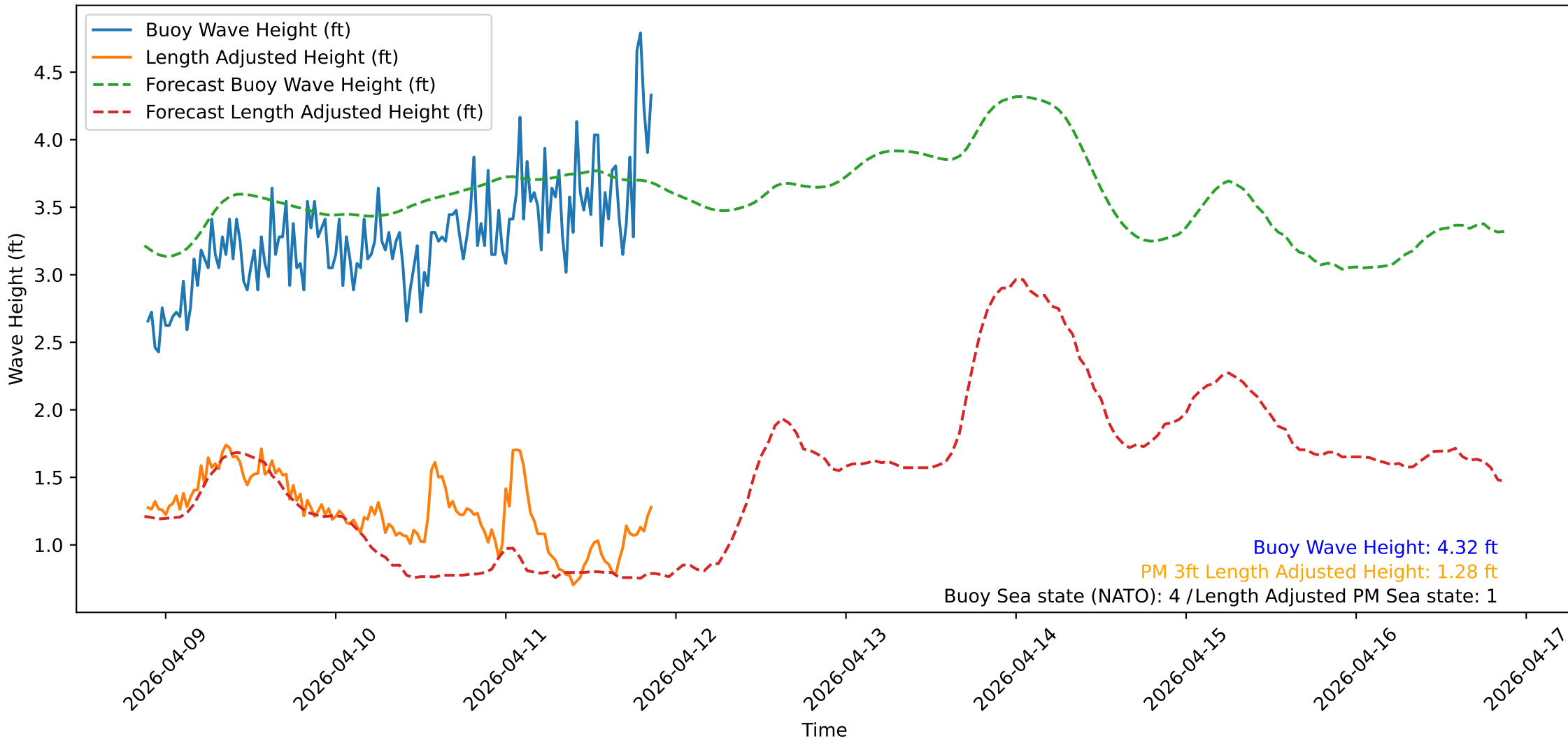
Wave Heights over Time for Oceanside Harbor at 2026-04-11 21:20:32
