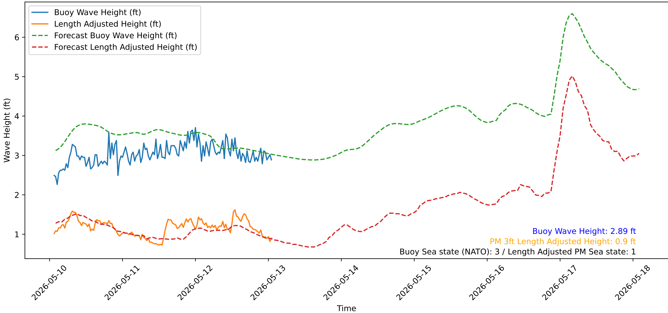
Wave Heights over Time for Oceanside Harbor at 2026-05-13 01:40:31
