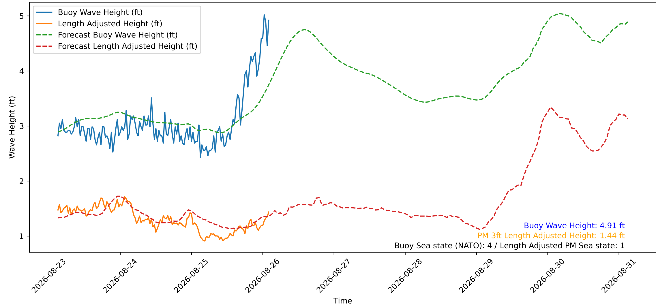
Wave Heights over Time for Oceanside Harbor at 2026-08-26 02:50:29
