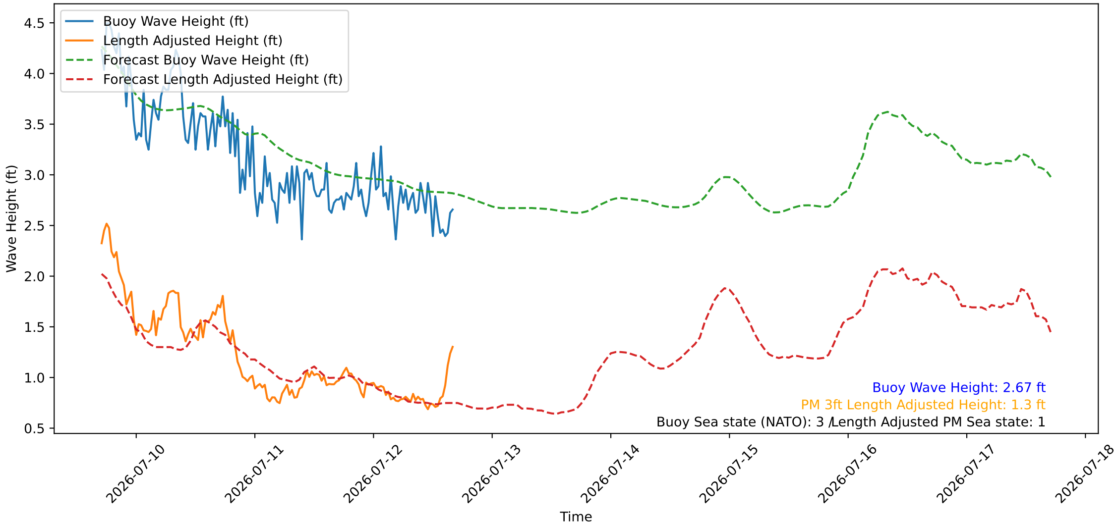
Wave Heights over Time for Oceanside Harbor at 2026-07-12 17:00:26
