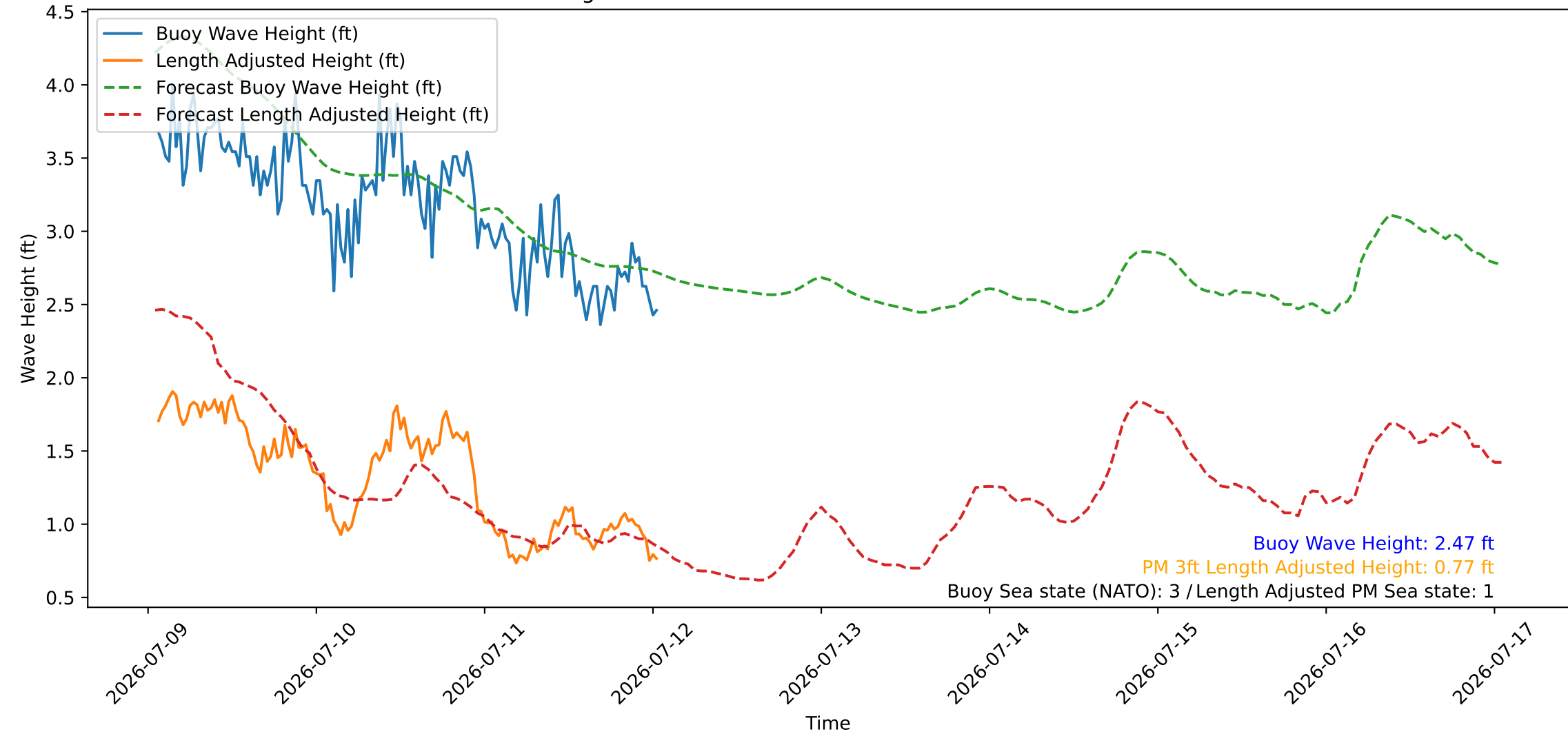
Wave Heights over Time for Red Beach at 2026-07-12 01:20:47
