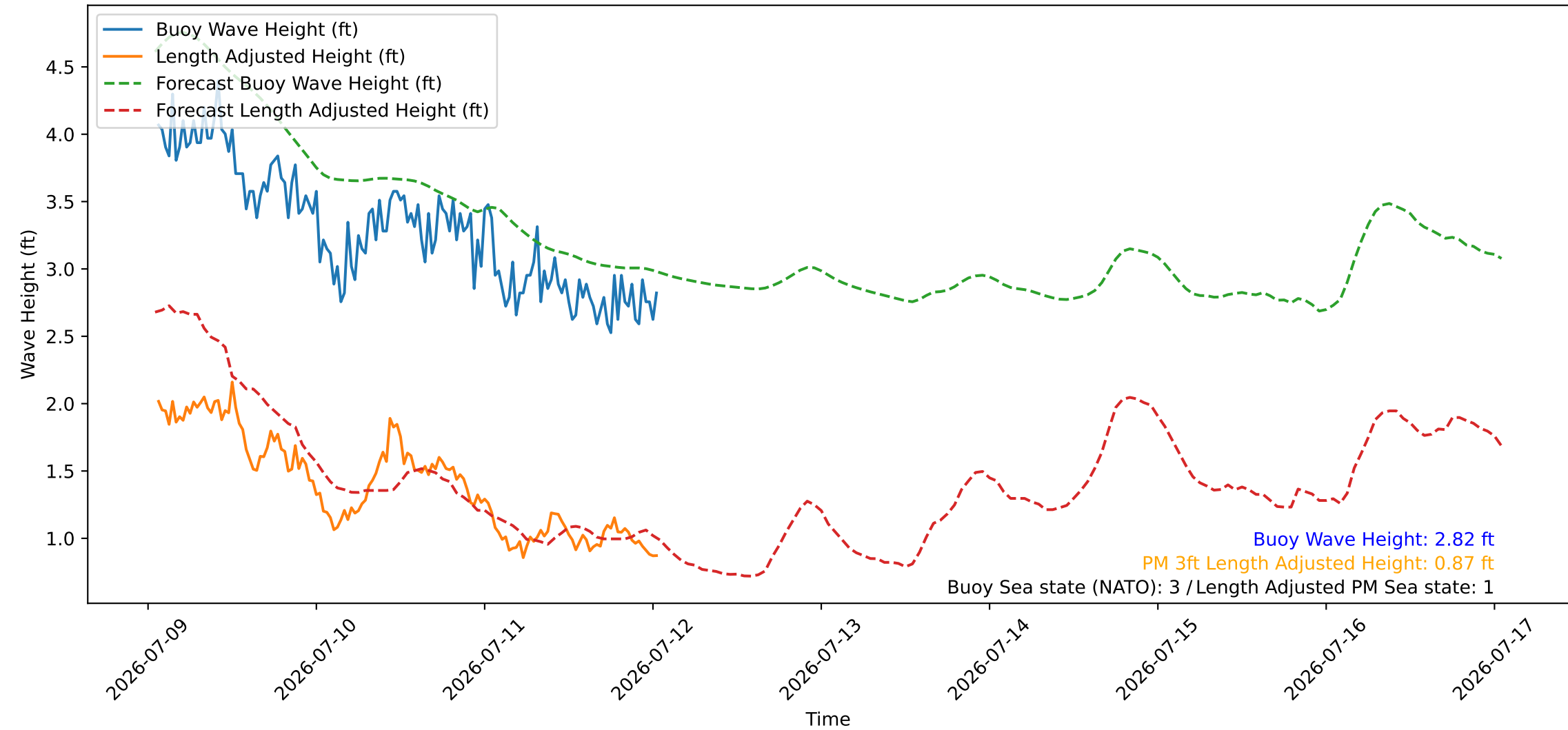
Wave Heights over Time for Green Beach at 2026-07-12 01:21:10
