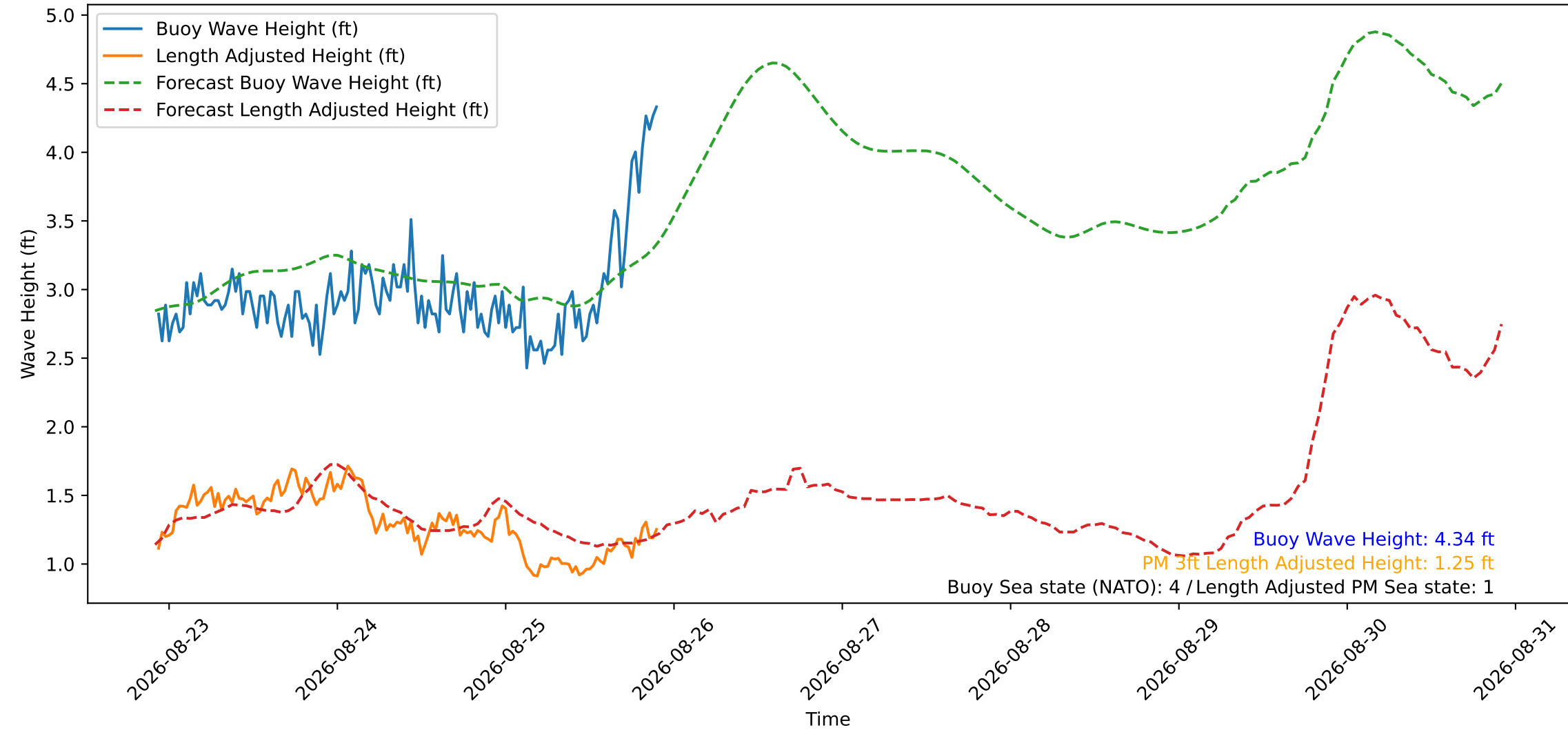
Wave Heights over Time for Oceanside Harbor at 2026-08-25 22:20:30
