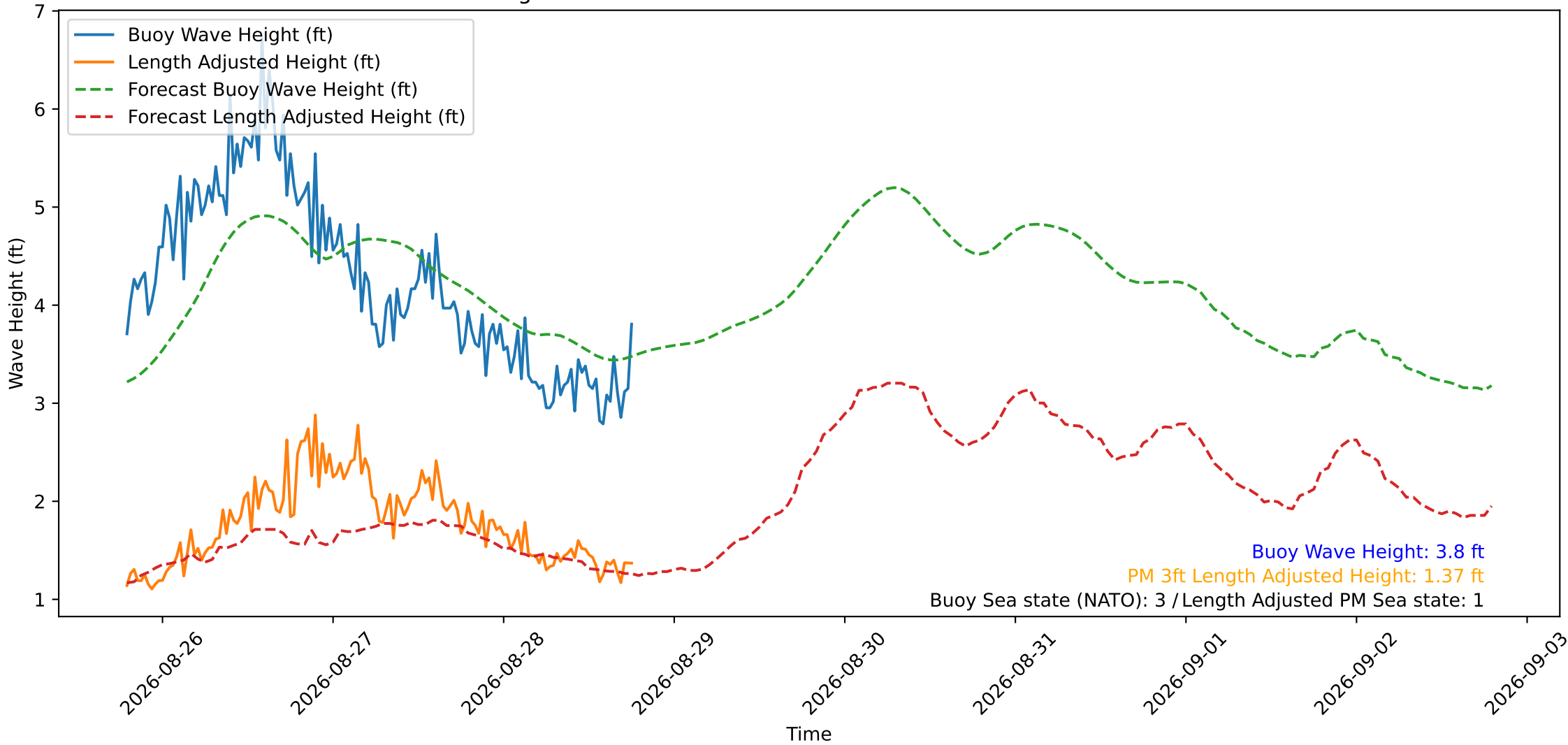
Wave Heights over Time for Oceanside Harbor at 2026-08-28 18:50:31
