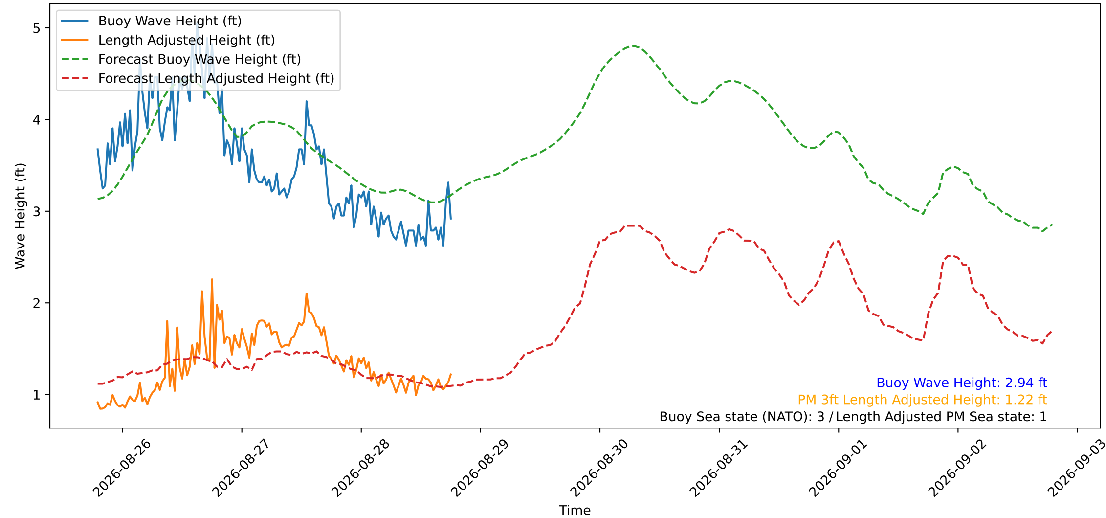
Wave Heights over Time for Red Beach at 2026-08-28 18:50:52
