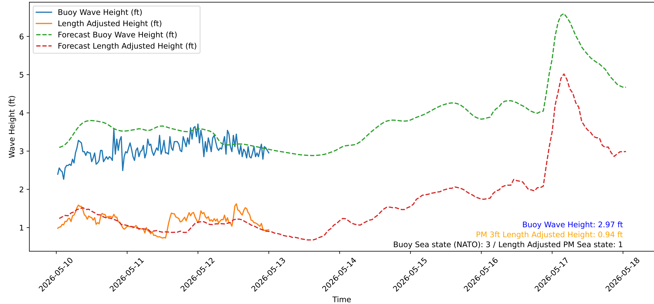
Wave Heights over Time for Oceanside Harbor at 2026-05-13 00:30:32
