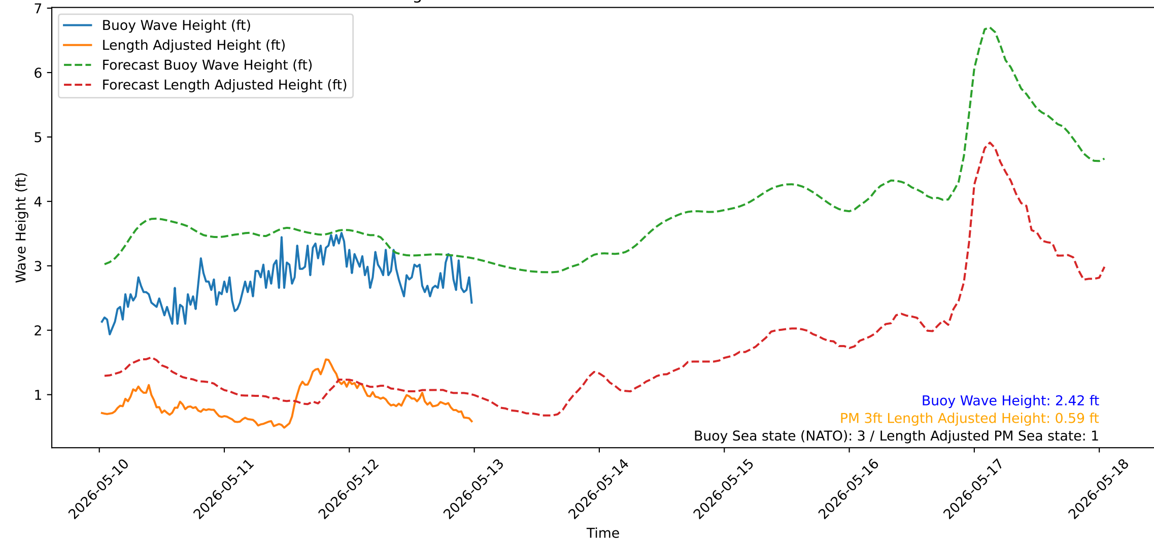
Wave Heights over Time for Green Beach at 2026-05-13 00:31:13
