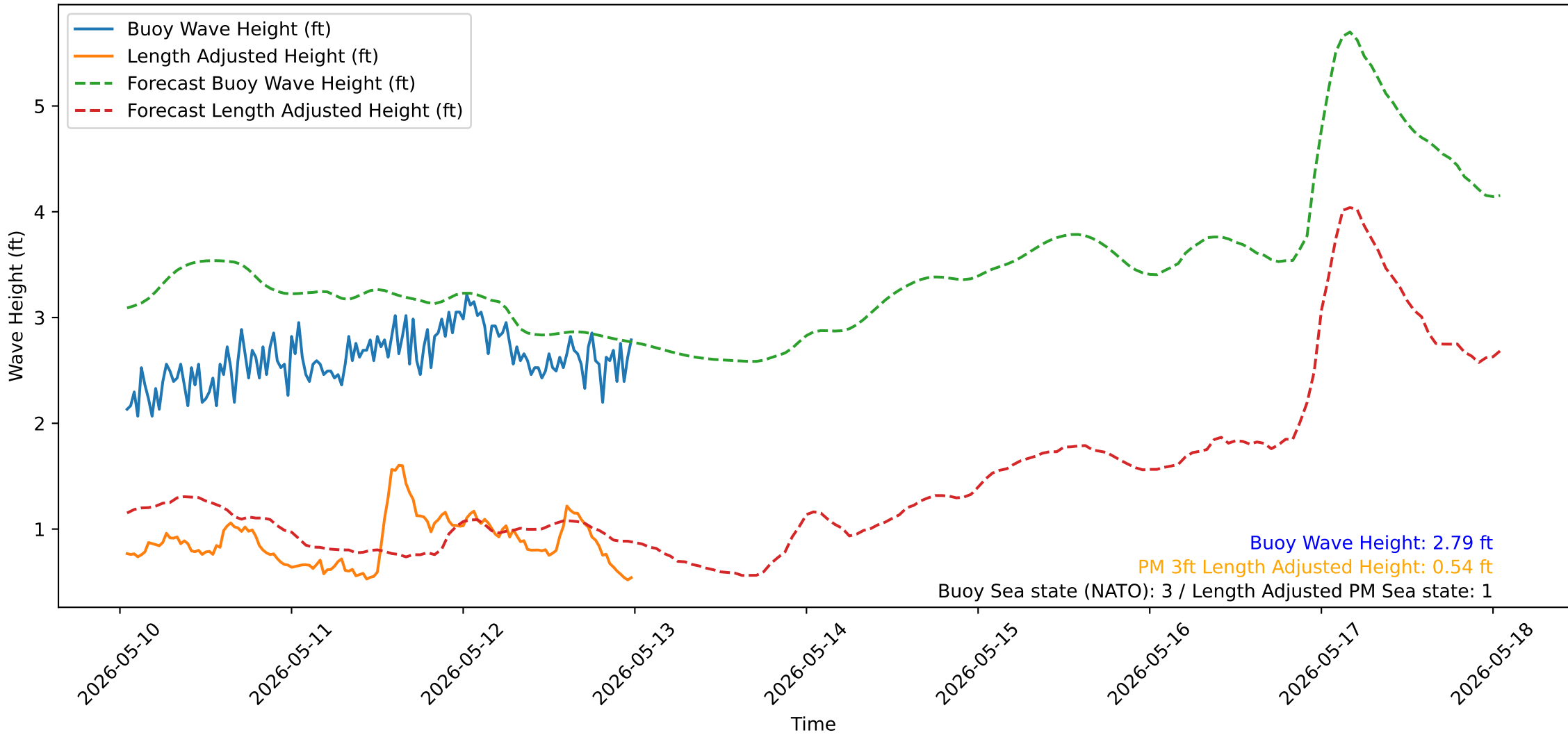
Wave Heights over Time for Red Beach at 2026-05-13 00:30:51
