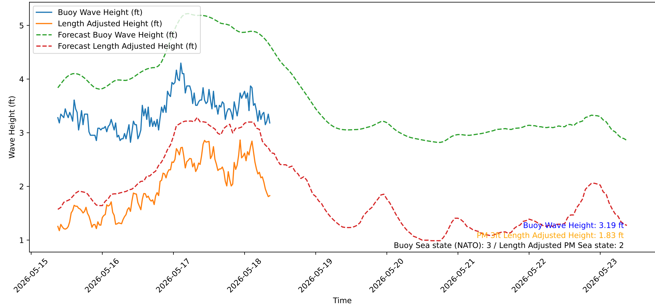
Wave Heights over Time for Oceanside Harbor at 2026-05-18 09:10:31
