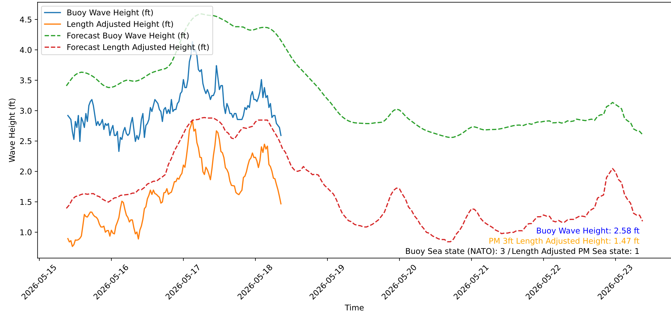
Wave Heights over Time for Red Beach at 2026-05-18 09:10:50
