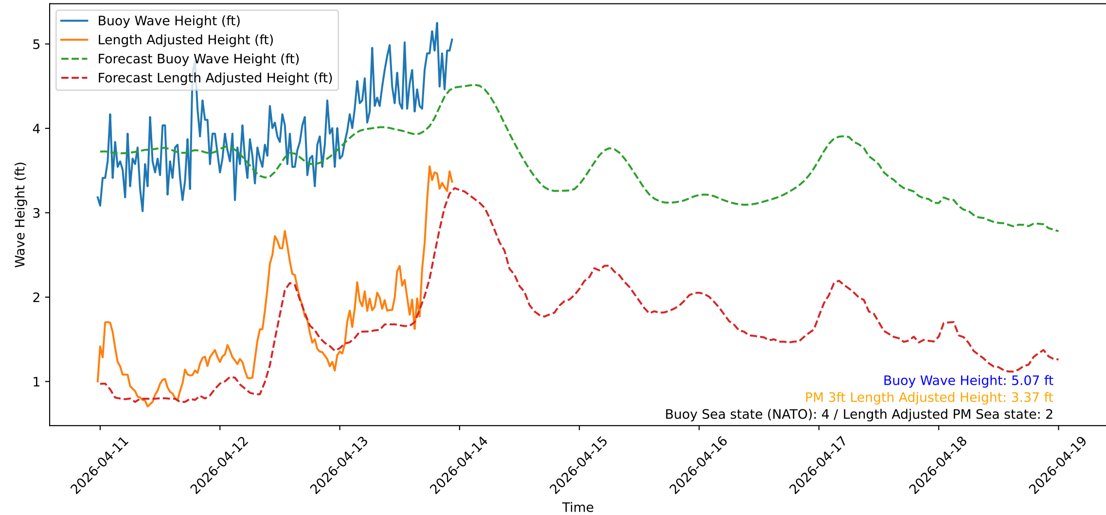
Wave Heights over Time for Oceanside Harbor at 2026-04-13 23:30:31
