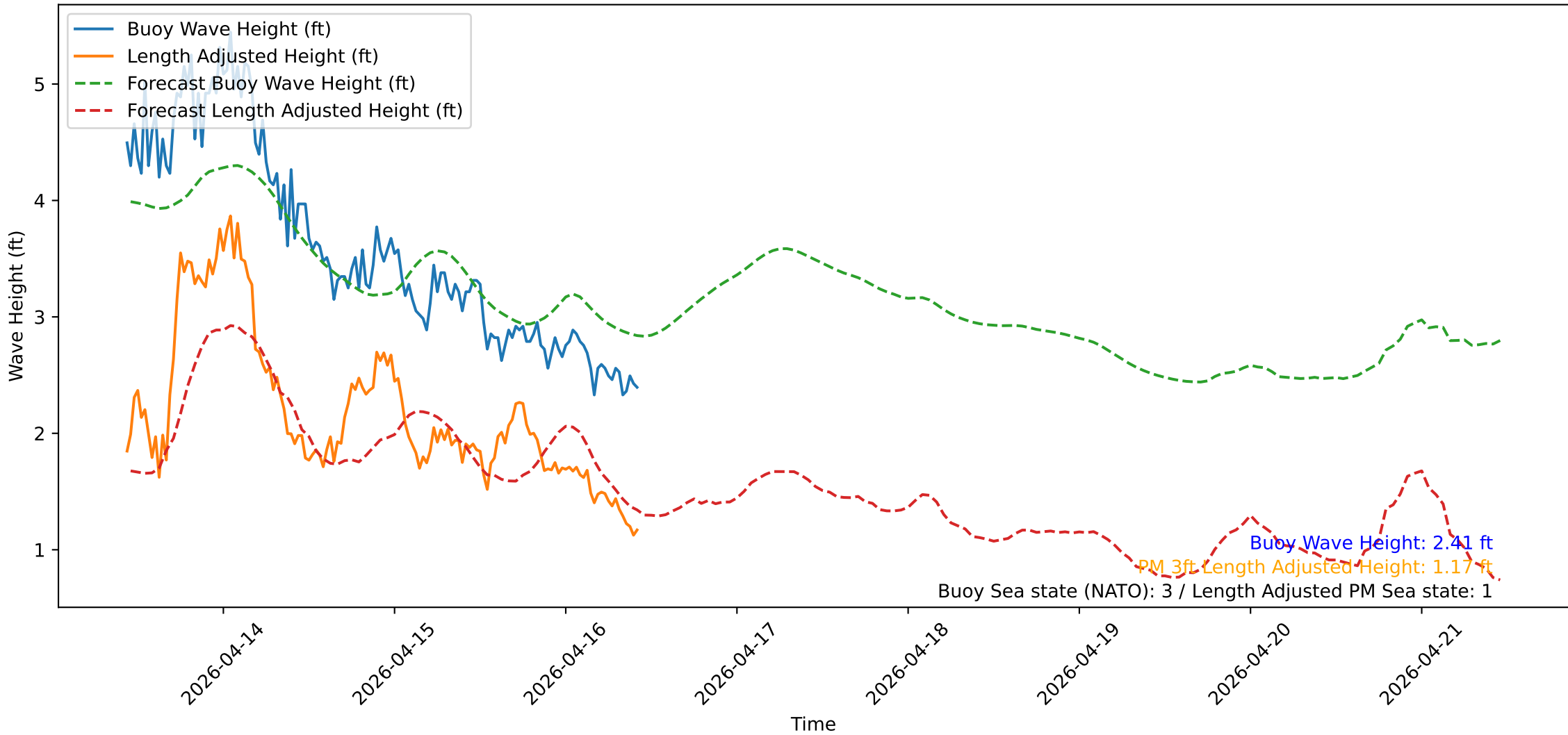
Wave Heights over Time for Oceanside Harbor at 2026-04-16 10:40:31
