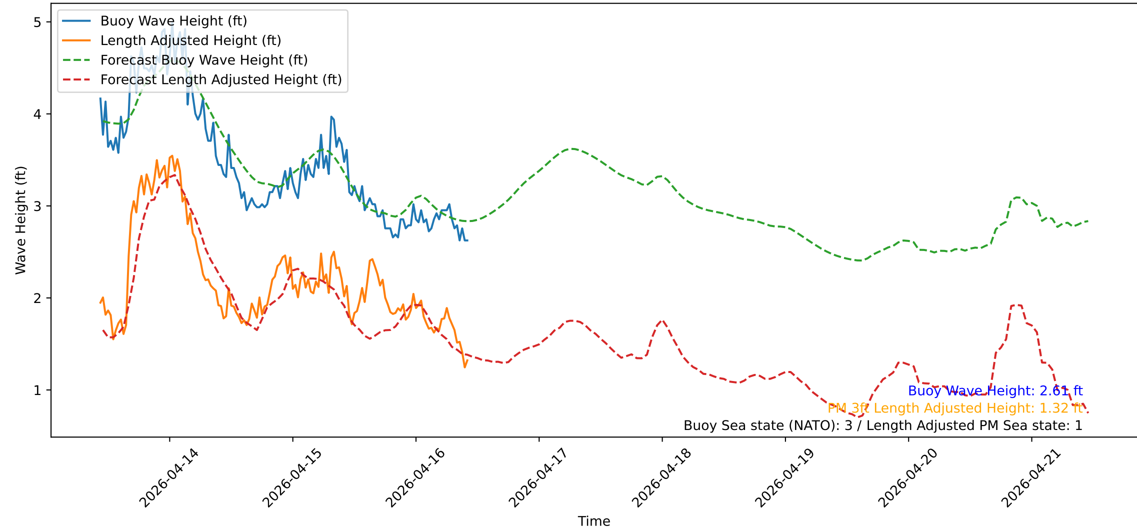
Wave Heights over Time for Green Beach at 2026-04-16 10:41:13
