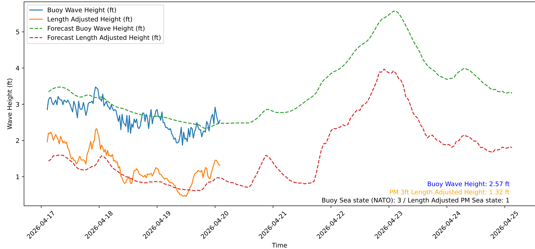
Wave Heights over Time for Green Beach at 2026-04-20 02:41:13
