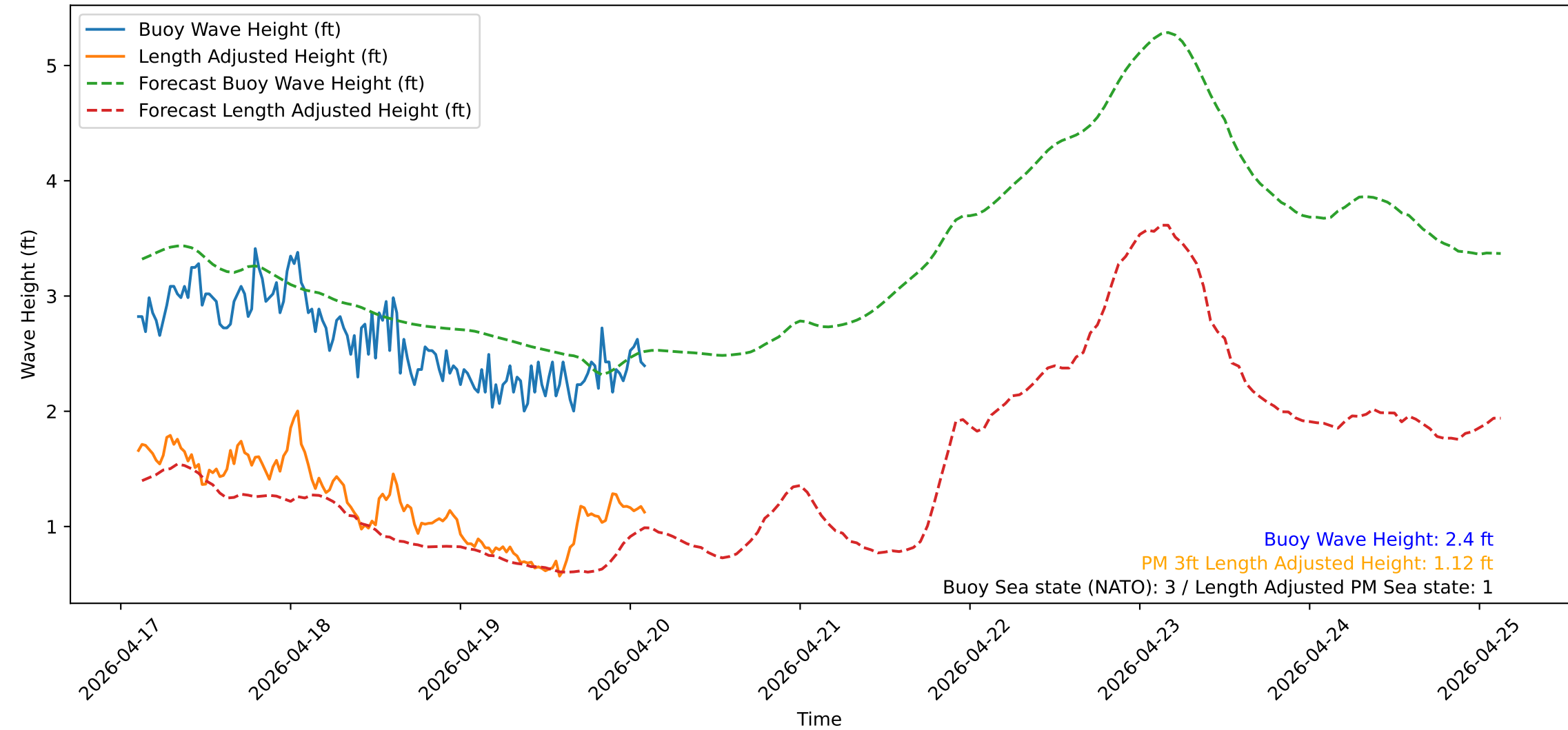
Wave Heights over Time for Oceanside Harbor at 2026-04-20 02:40:31
