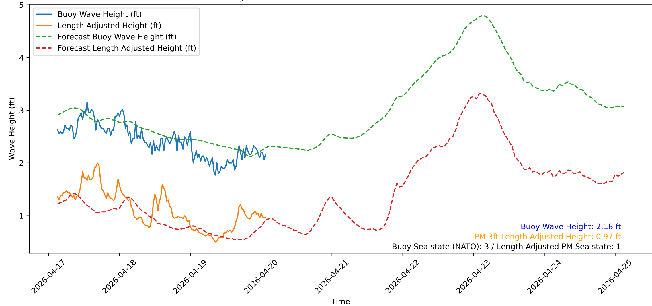
Wave Heights over Time for Red Beach at 2026-04-20 02:40:50
