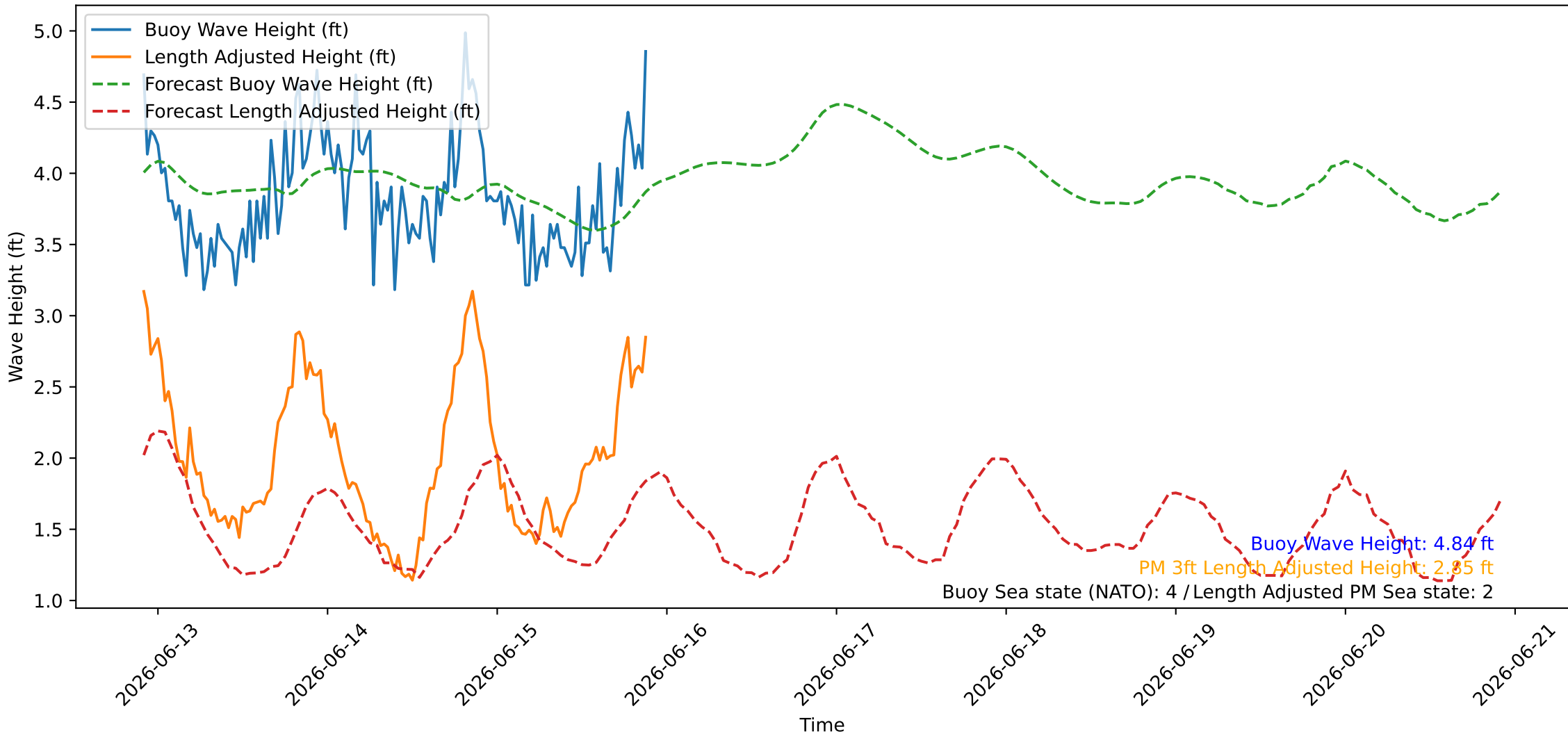
Wave Heights over Time for Oceanside Harbor at 2026-06-15 21:50:26
