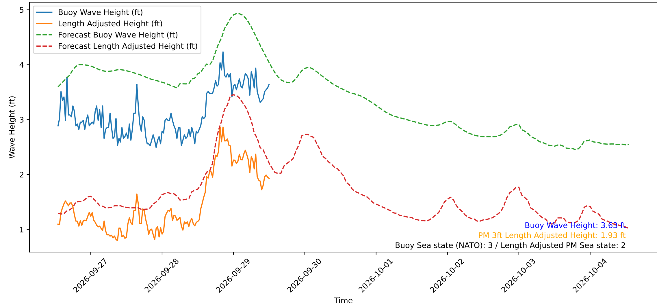
Wave Heights over Time for Oceanside Harbor at 2026-09-29 12:50:30
