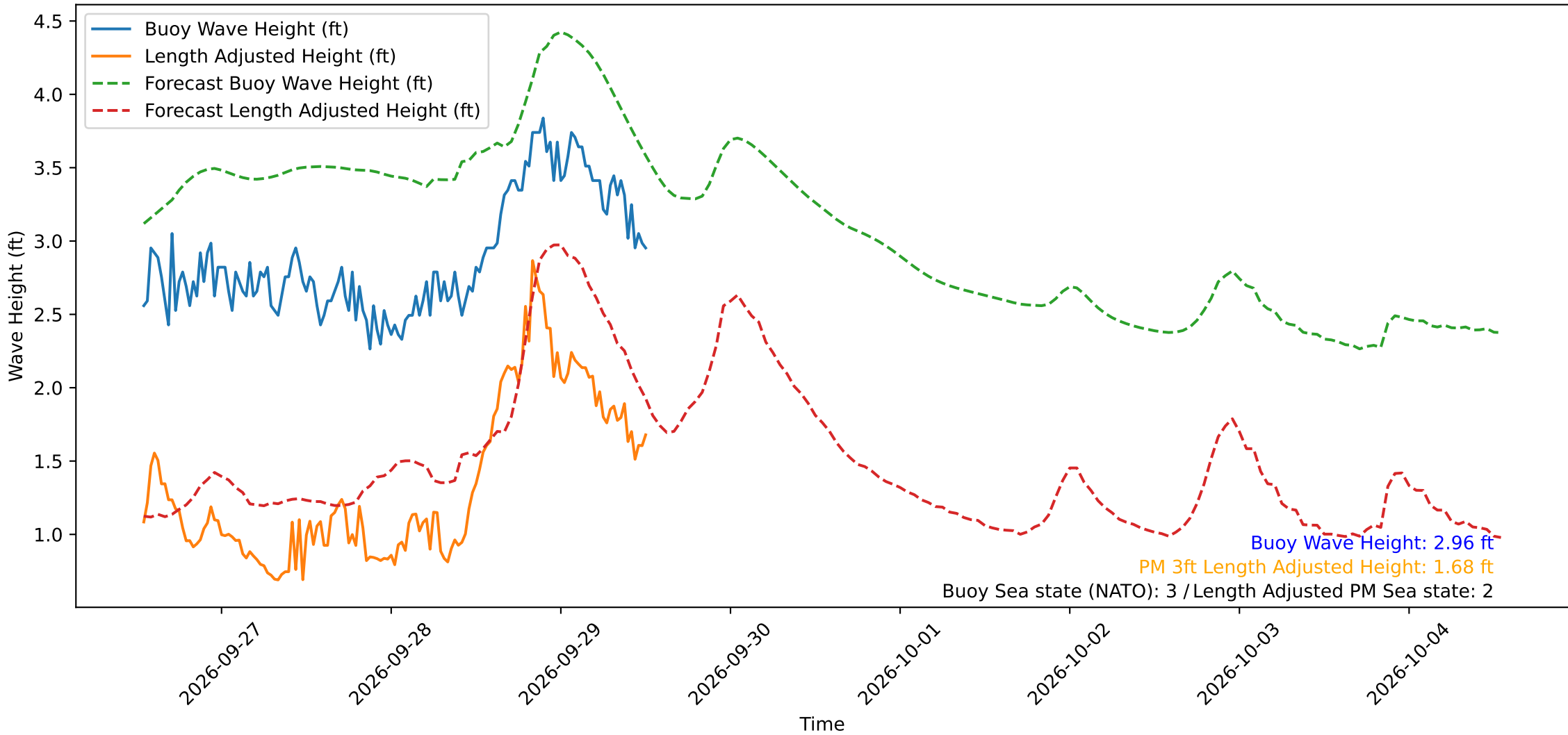
Wave Heights over Time for Red Beach at 2026-09-29 12:50:51
