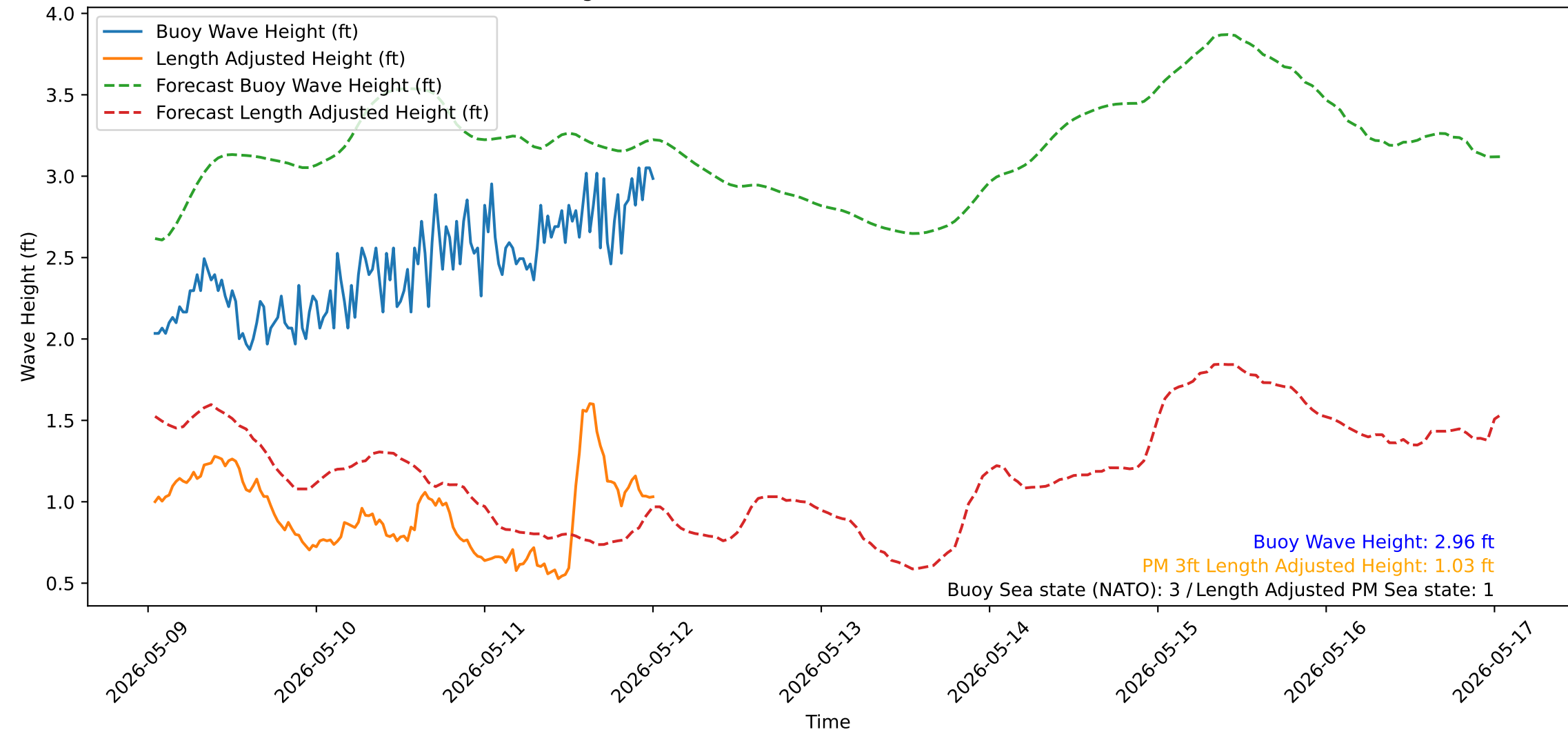
Wave Heights over Time for Red Beach at 2026-05-12 00:40:50
