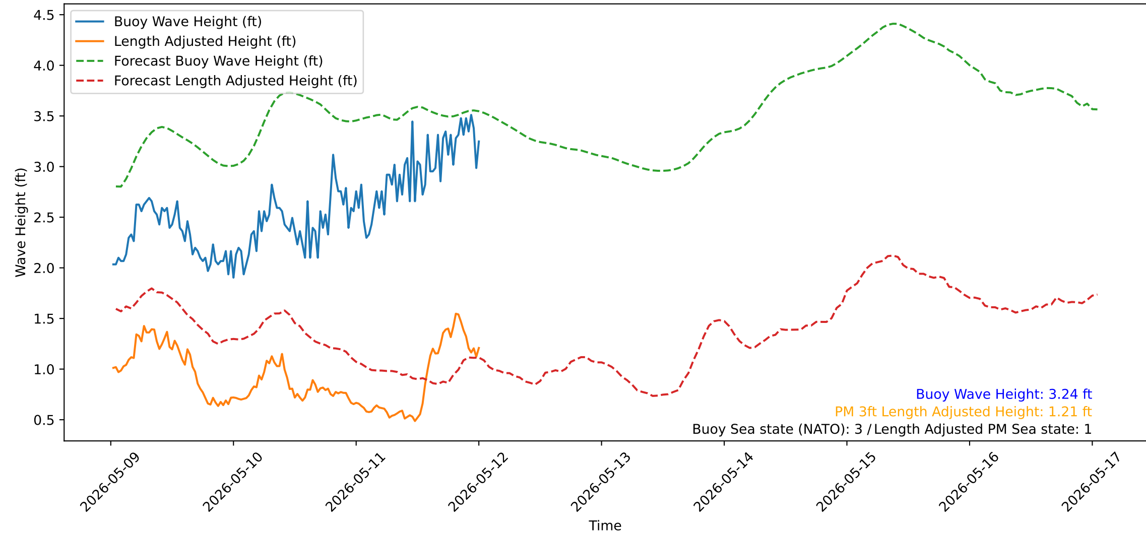
Wave Heights over Time for Green Beach at 2026-05-12 00:41:12
