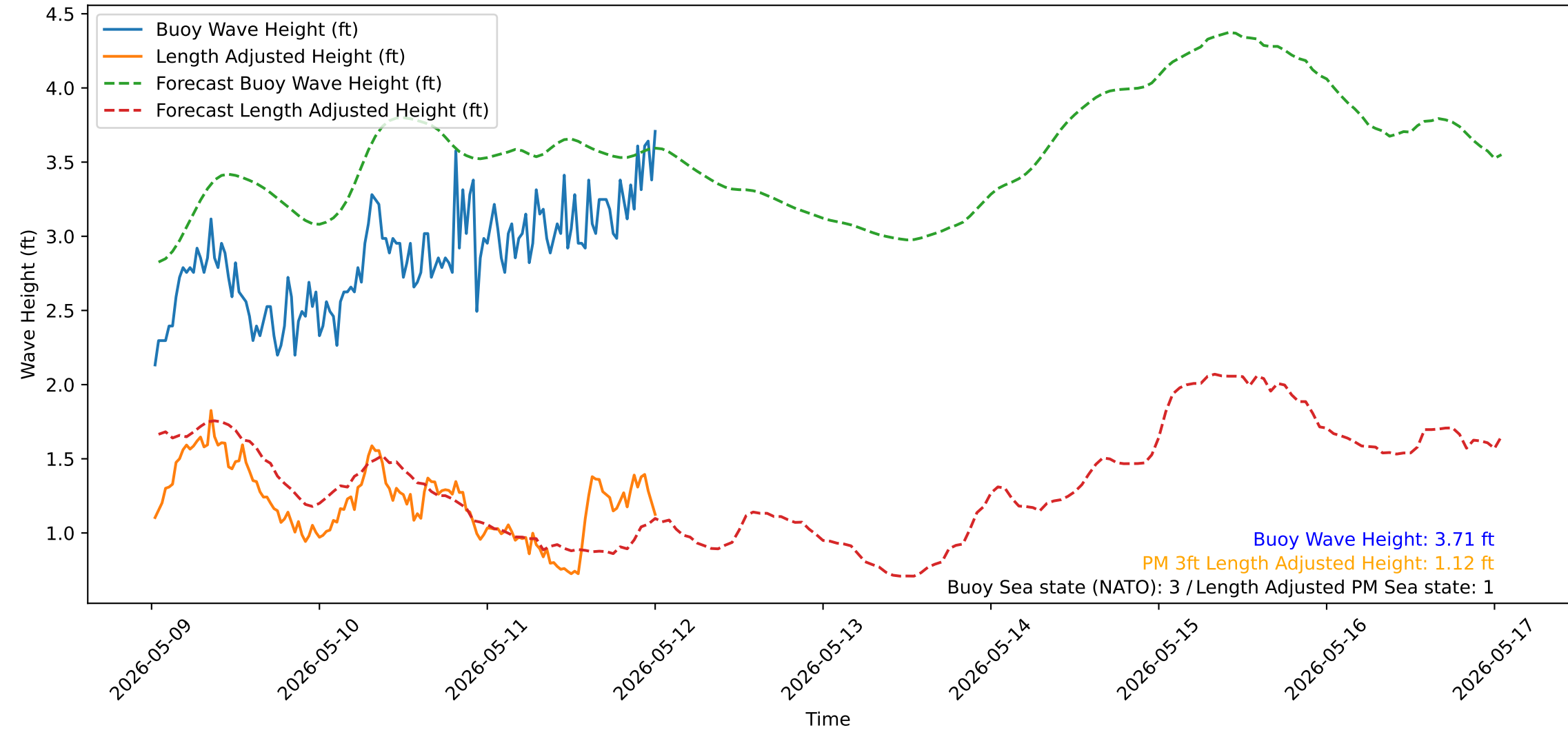
Wave Heights over Time for Oceanside Harbor at 2026-05-12 00:40:31
