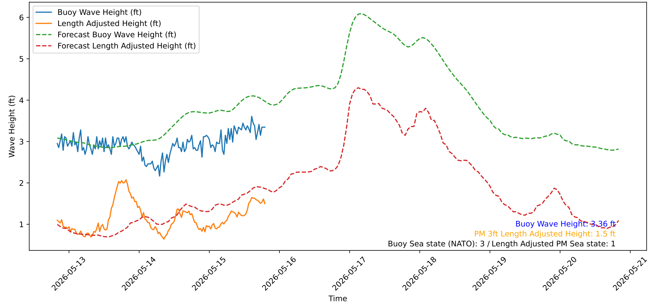
Wave Heights over Time for Oceanside Harbor at 2026-05-15 19:50:31
