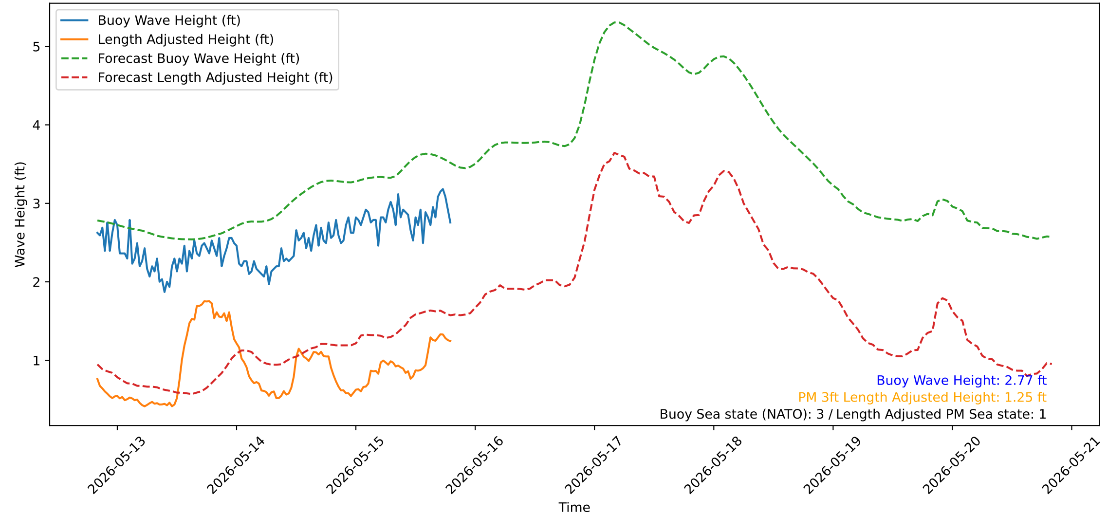
Wave Heights over Time for Red Beach at 2026-05-15 19:50:52
