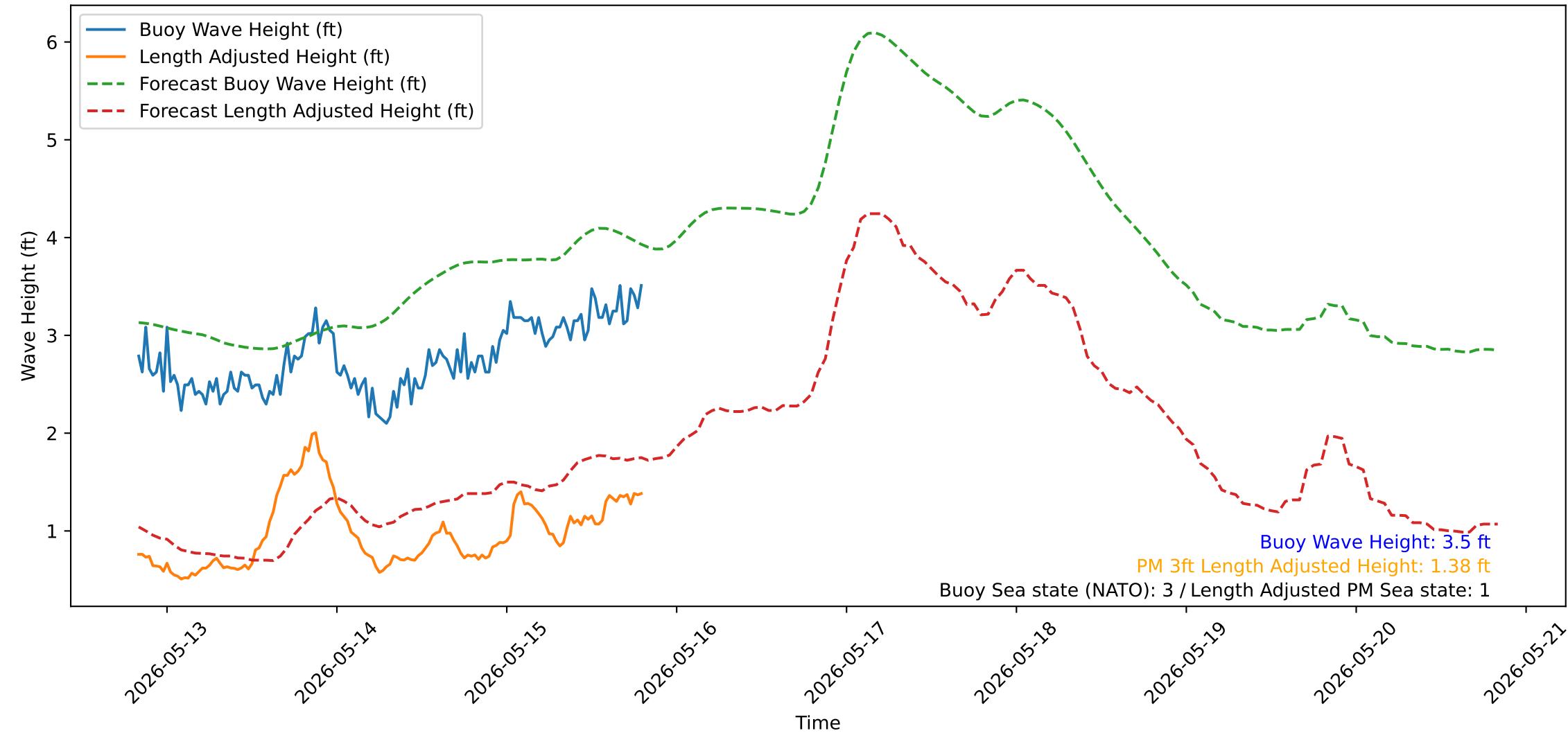
Wave Heights over Time for Green Beach at 2026-05-15 19:51:14
