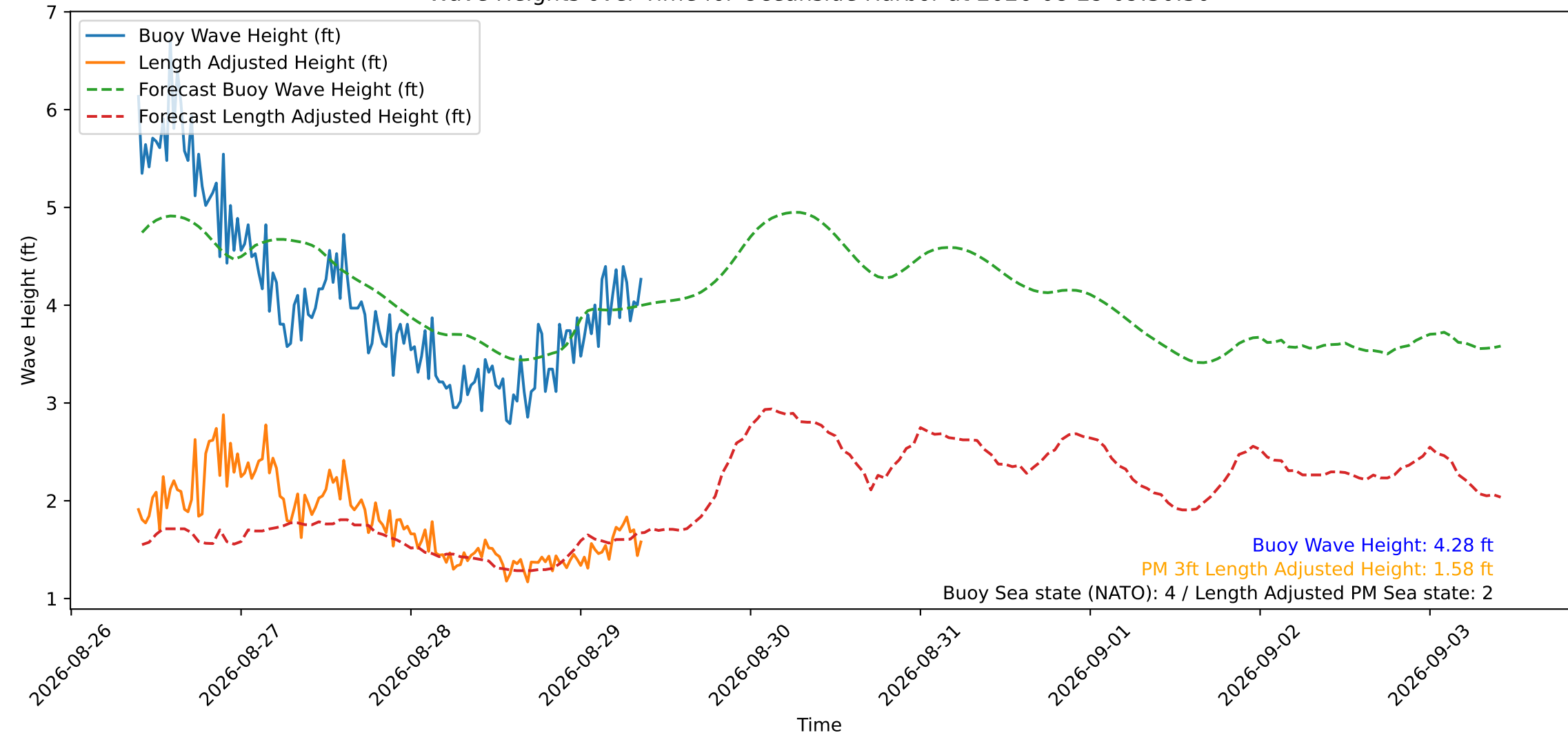
Wave Heights over Time for Oceanside Harbor at 2026-08-29 09:30:30
