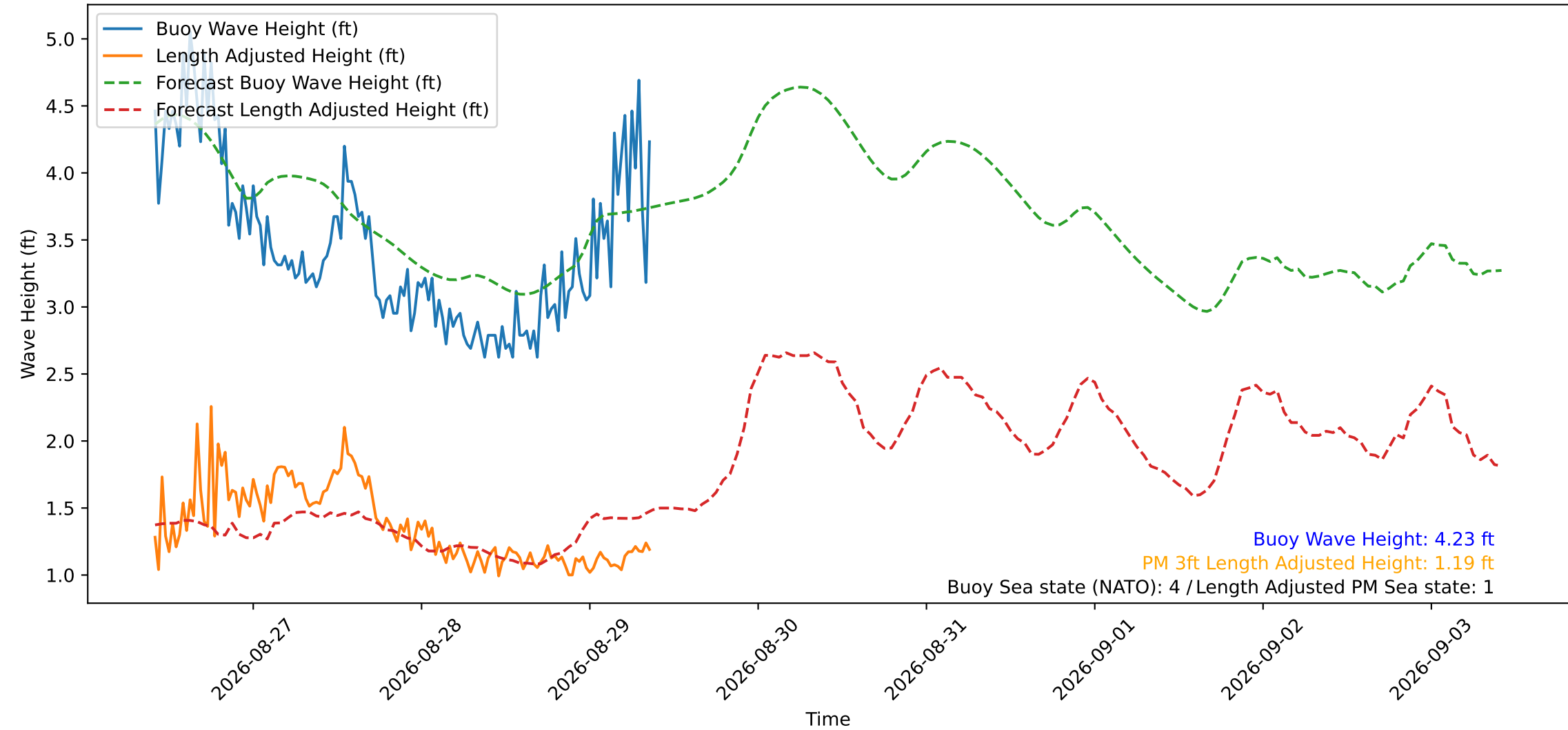
Wave Heights over Time for Red Beach at 2026-08-29 09:30:50
