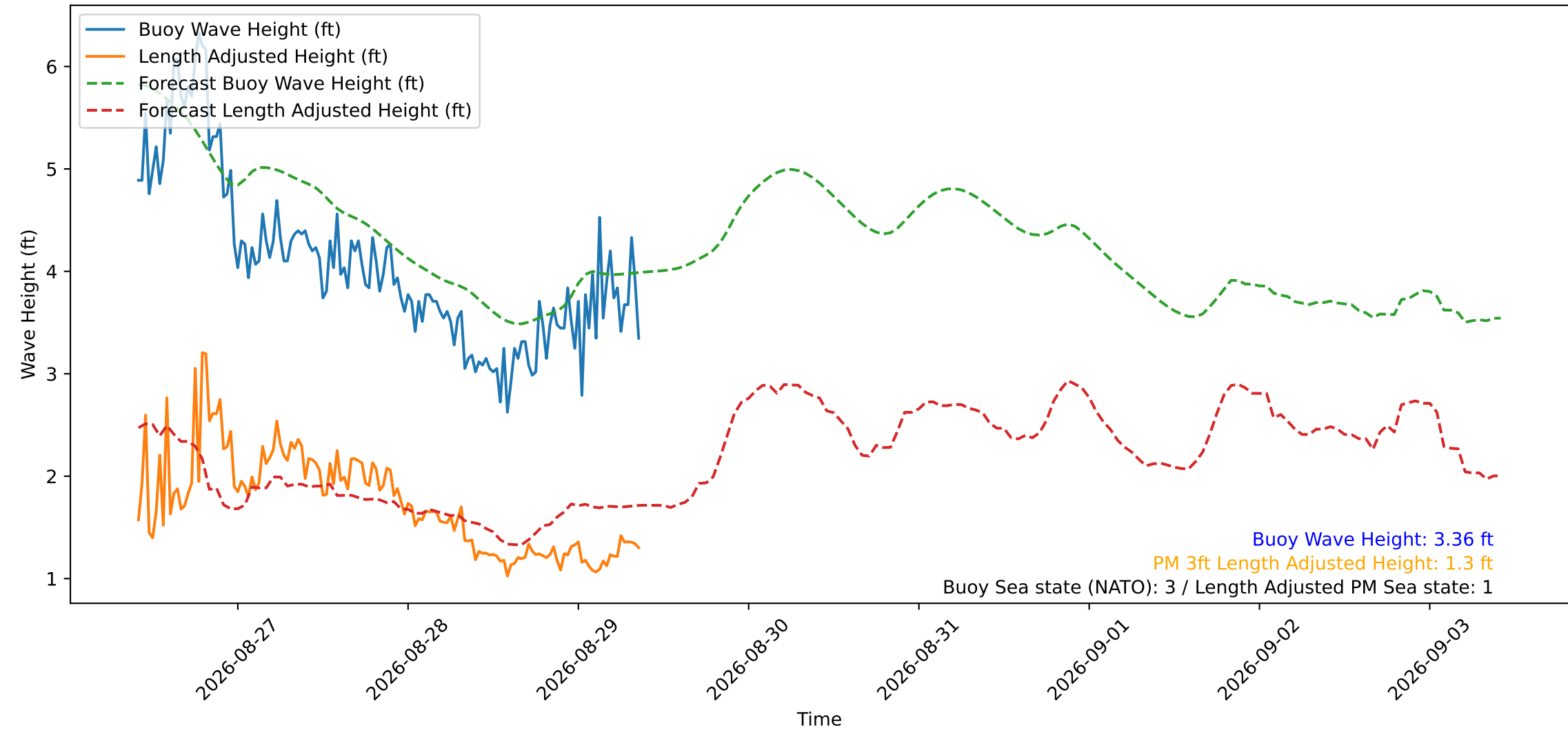
Wave Heights over Time for Green Beach at 2026-08-29 09:31:12
