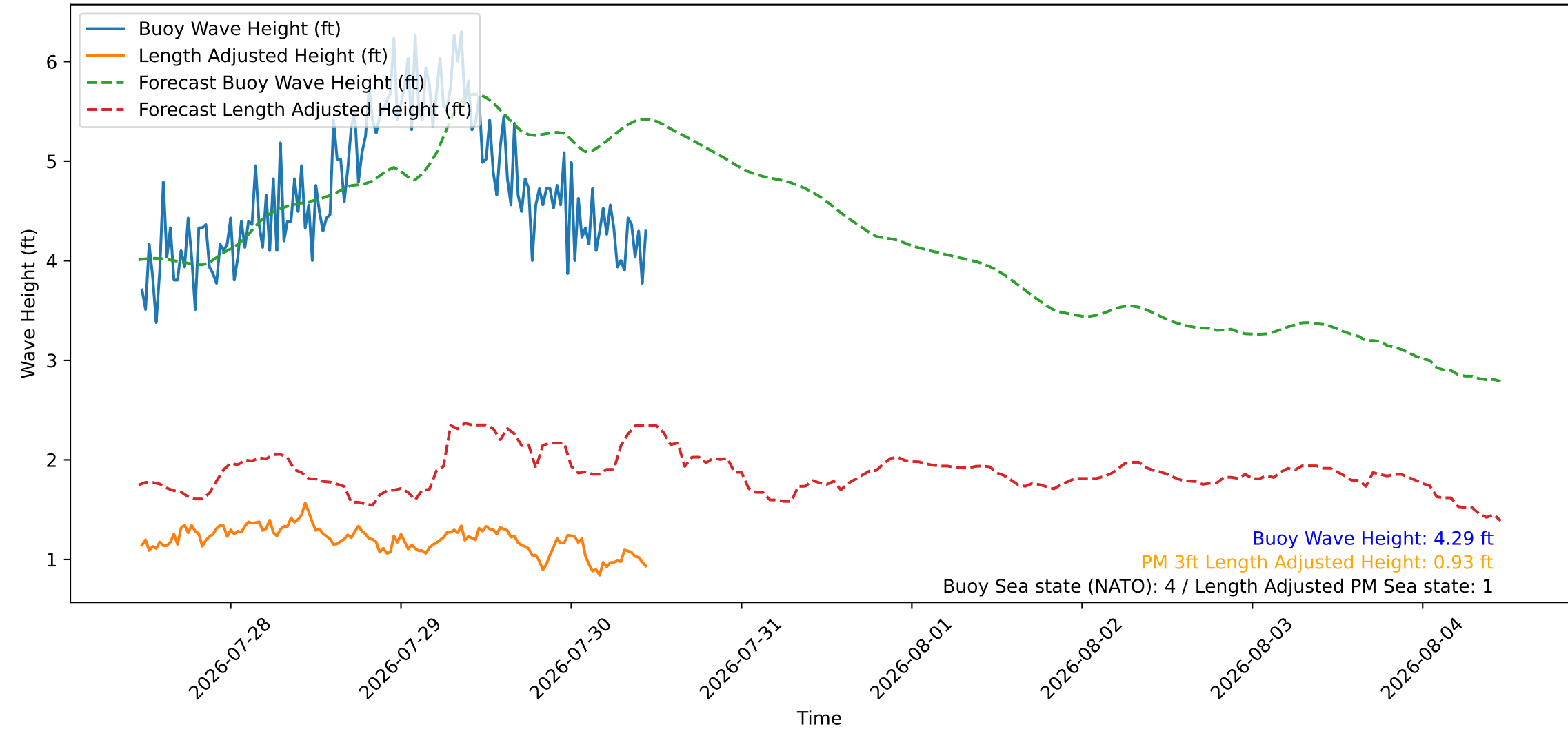
Wave Heights over Time for Green Beach at 2026-07-30 11:21:10
