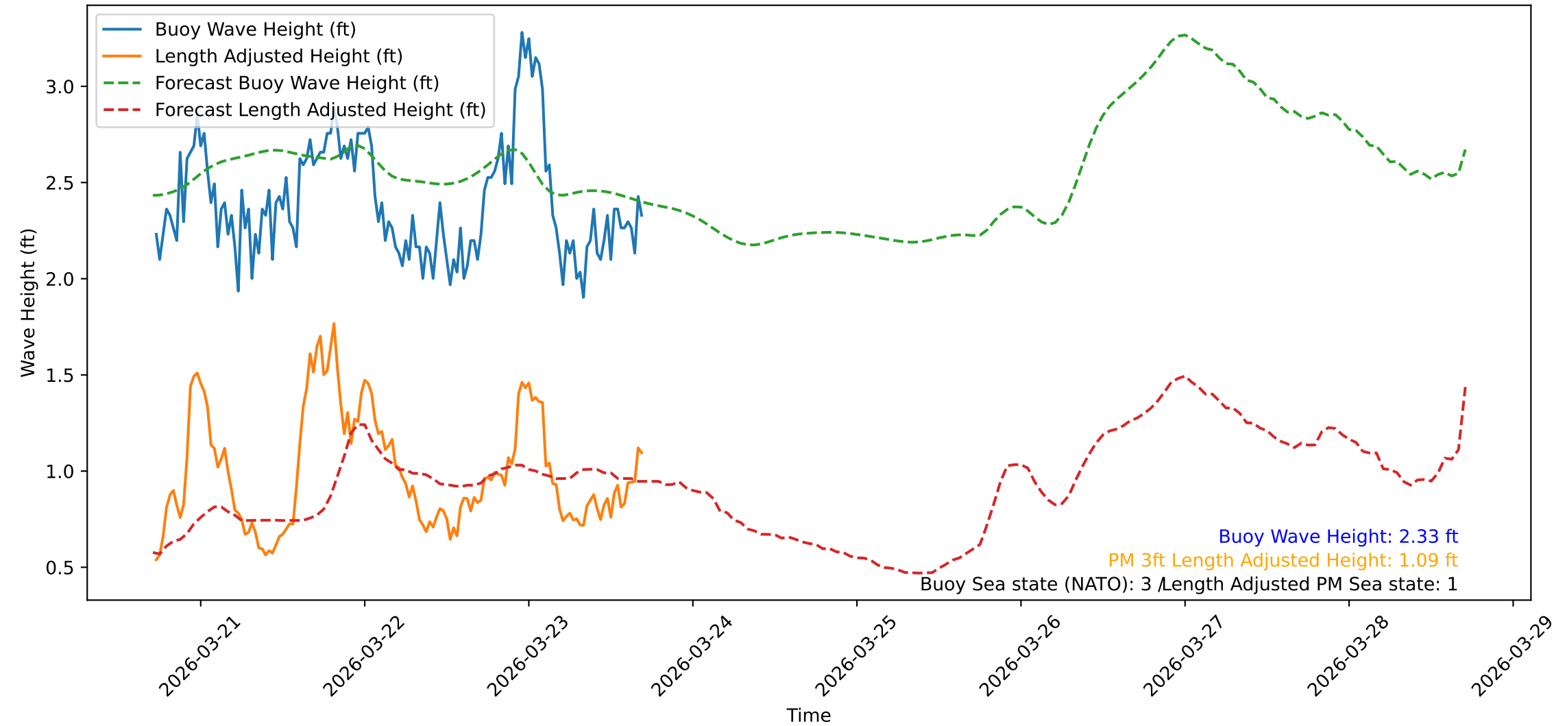
Wave Heights over Time for Green Beach at 2026-03-23 17:21:10
