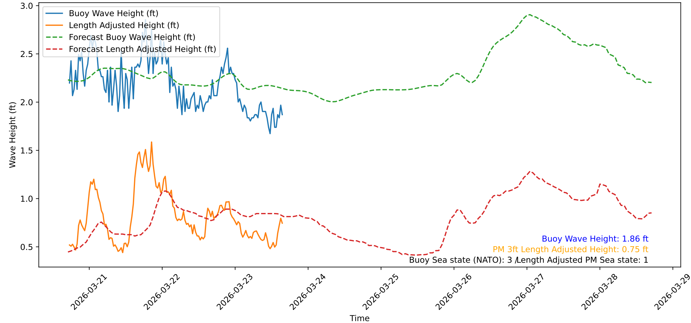
Wave Heights over Time for Red Beach at 2026-03-23 17:20:48
