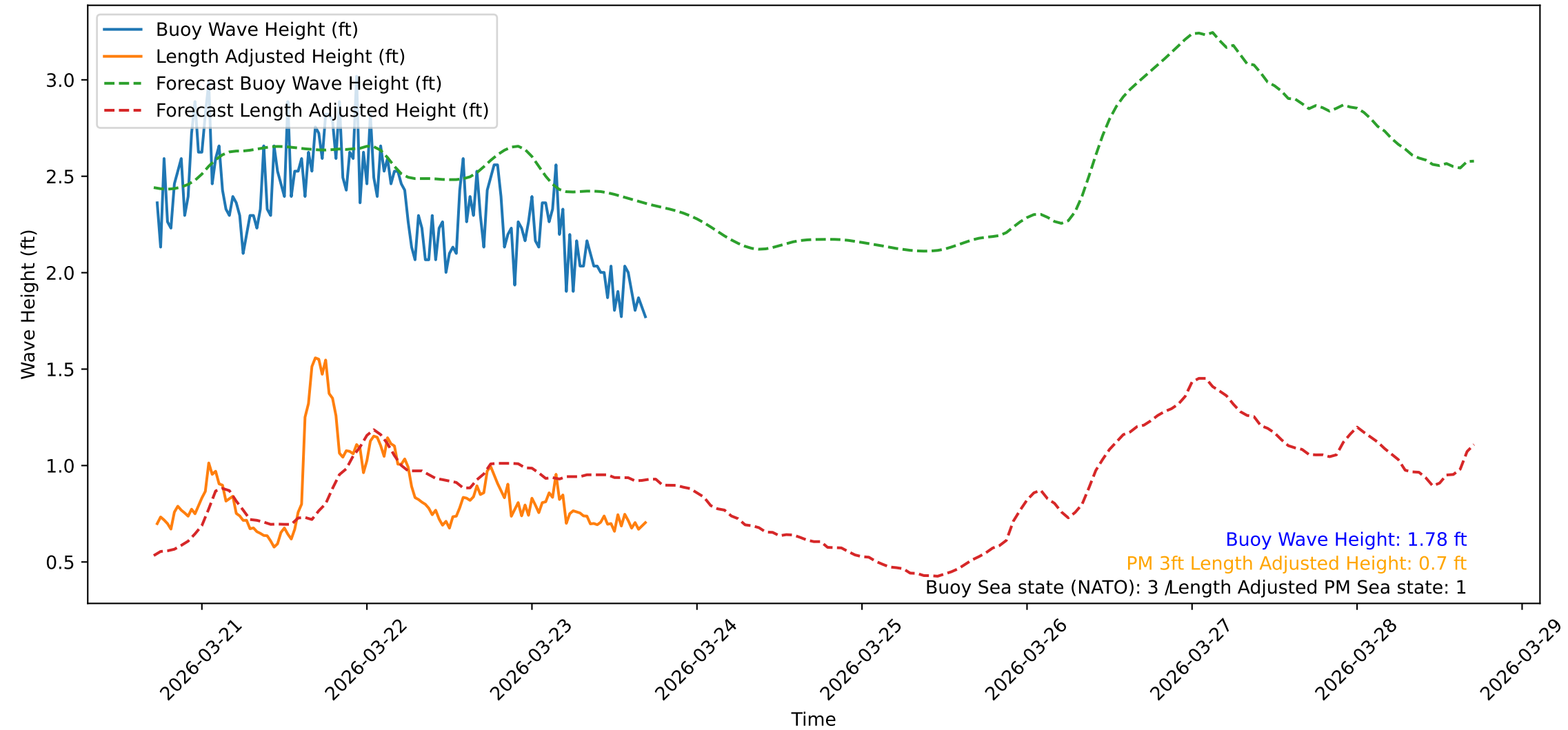
Wave Heights over Time for Oceanside Harbor at 2026-03-23 17:20:31
