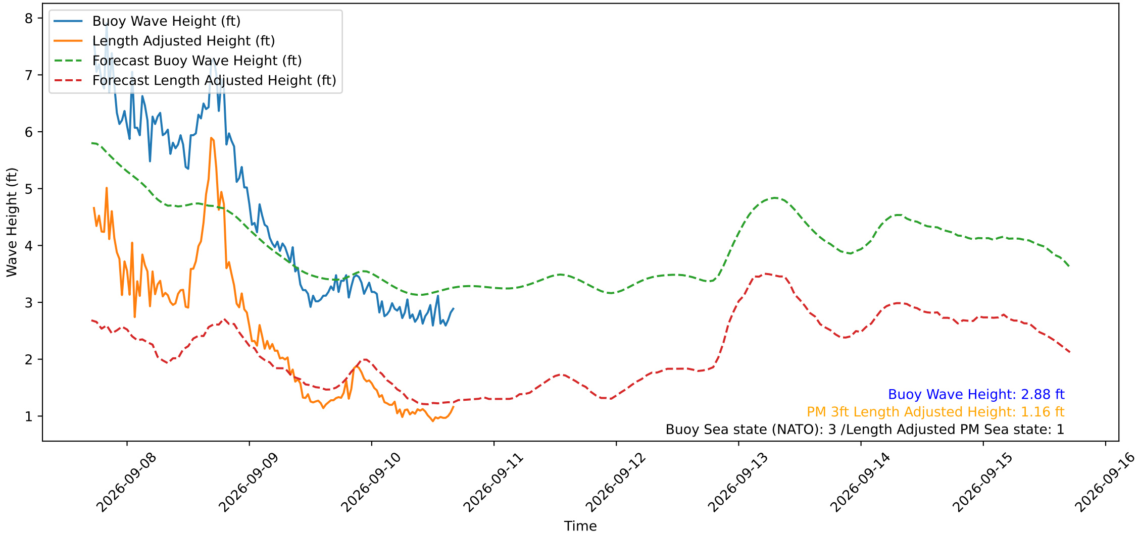
Wave Heights over Time for Green Beach at 2026-09-10 17:01:12
