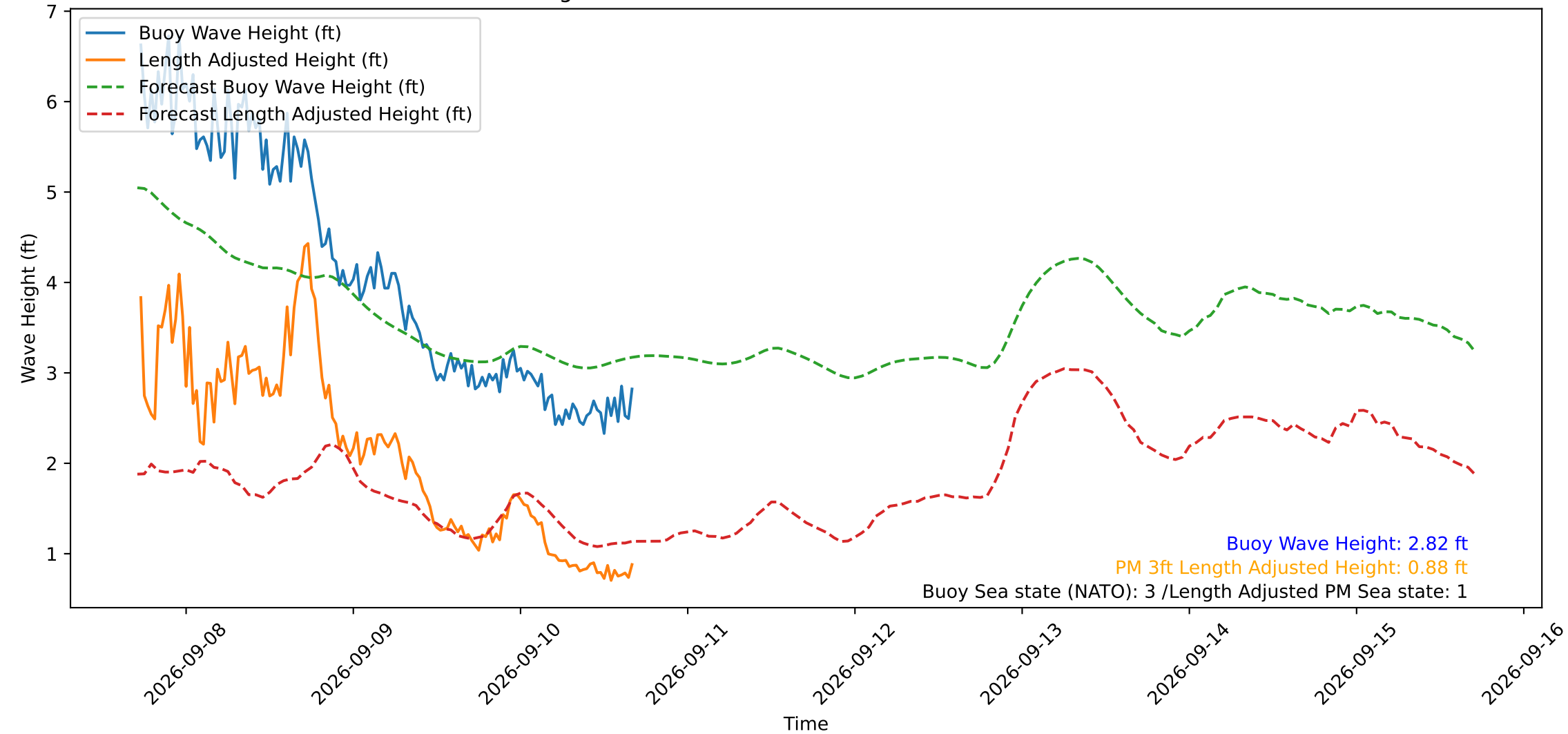
Wave Heights over Time for Red Beach at 2026-09-10 17:00:49
