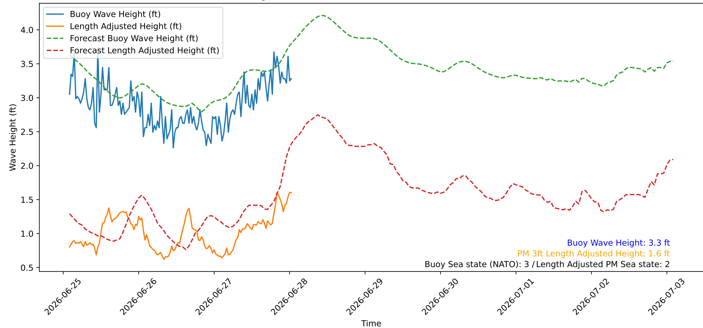
Wave Heights over Time for Red Beach at 2026-06-28 01:30:45
