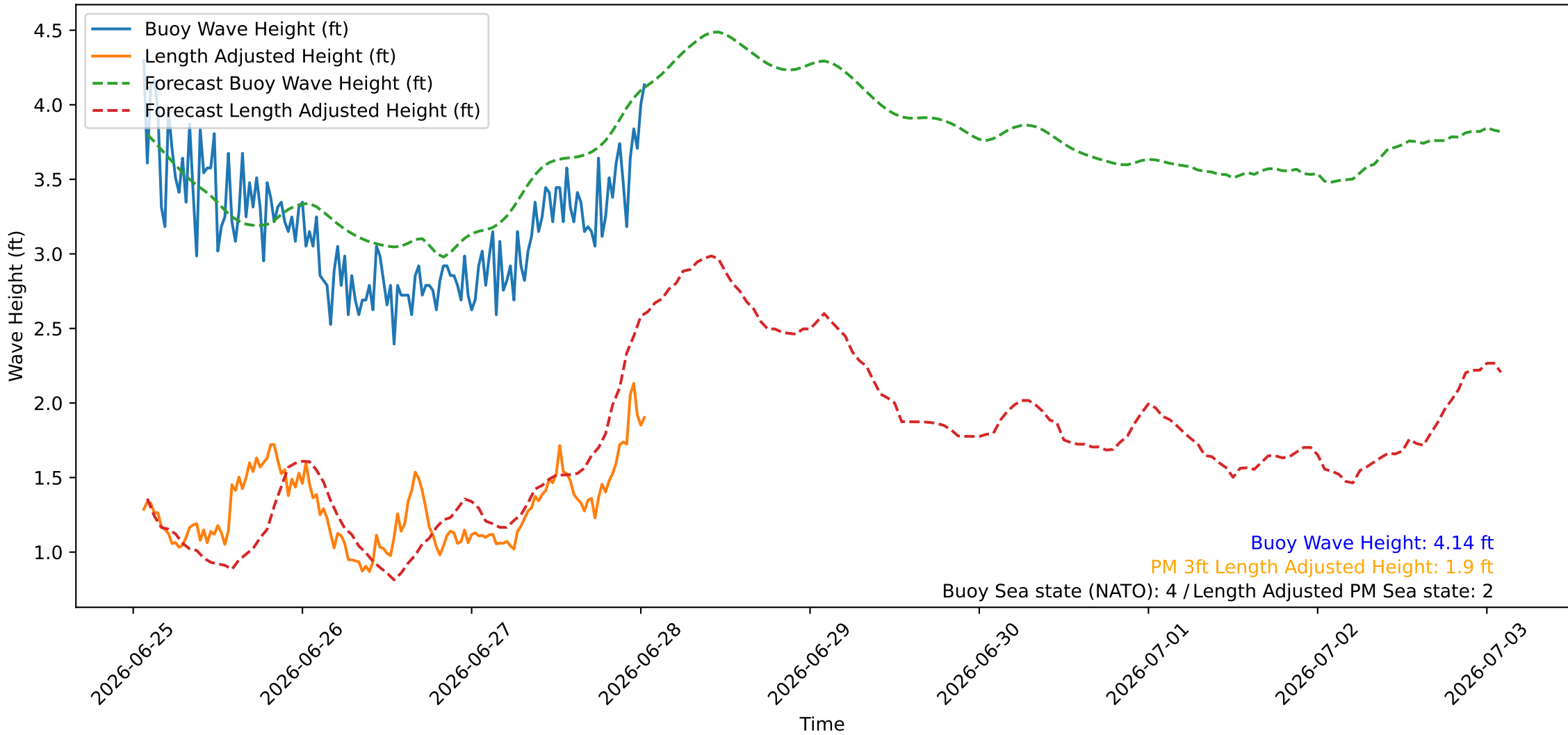
Wave Heights over Time for Oceanside Harbor at 2026-06-28 01:30:26
