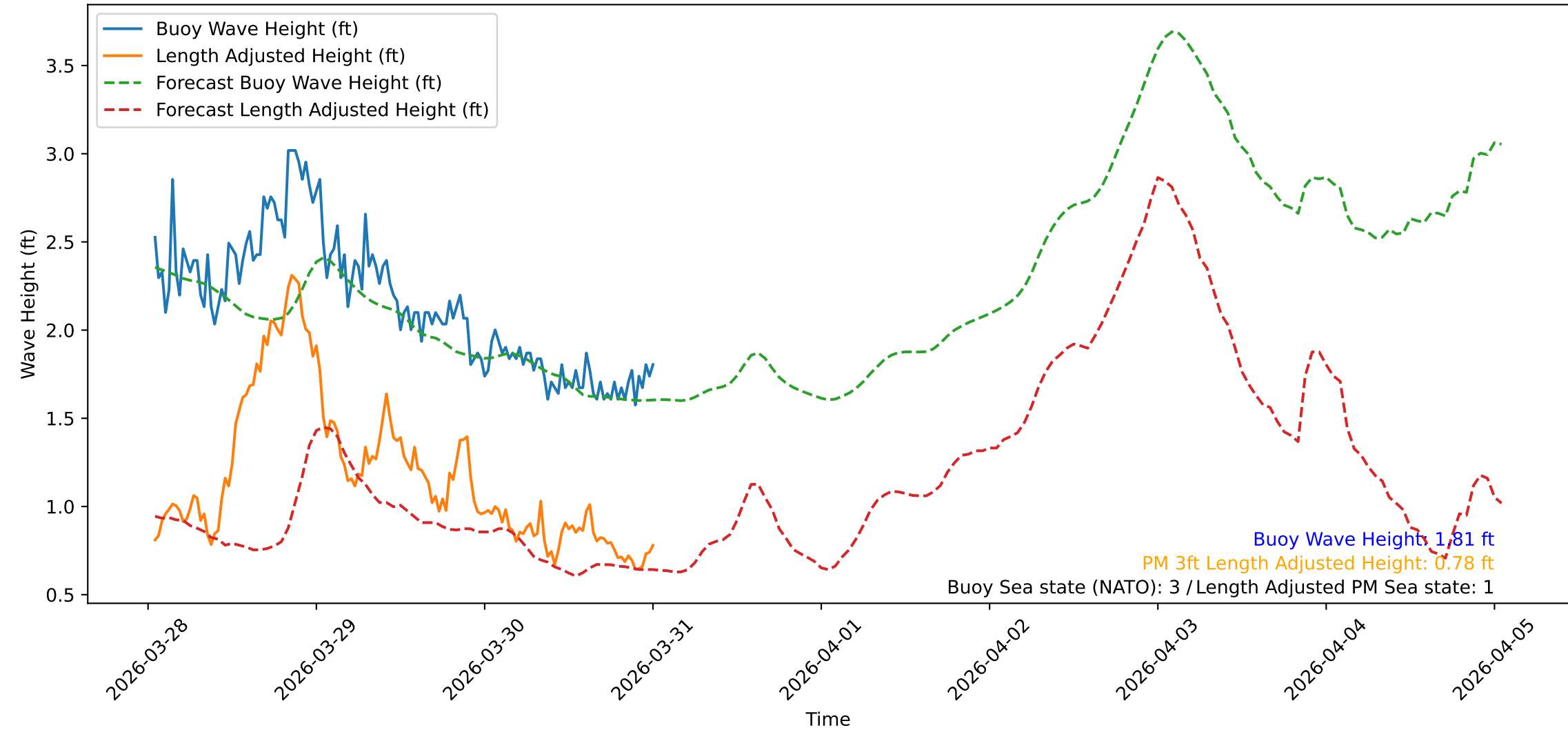
Wave Heights over Time for Red Beach at 2026-03-31 00:50:47
