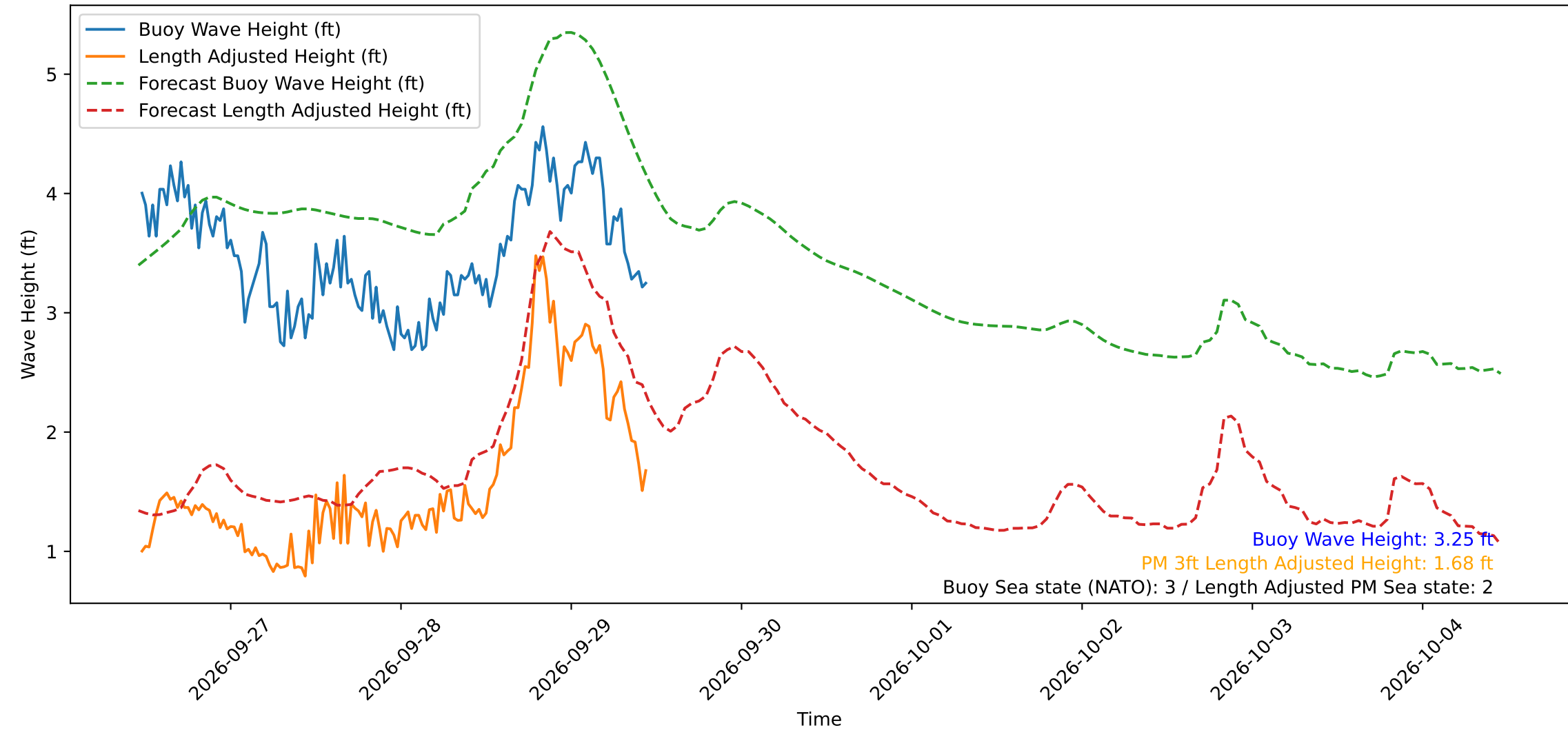
Wave Heights over Time for Green Beach at 2026-09-29 11:21:16
