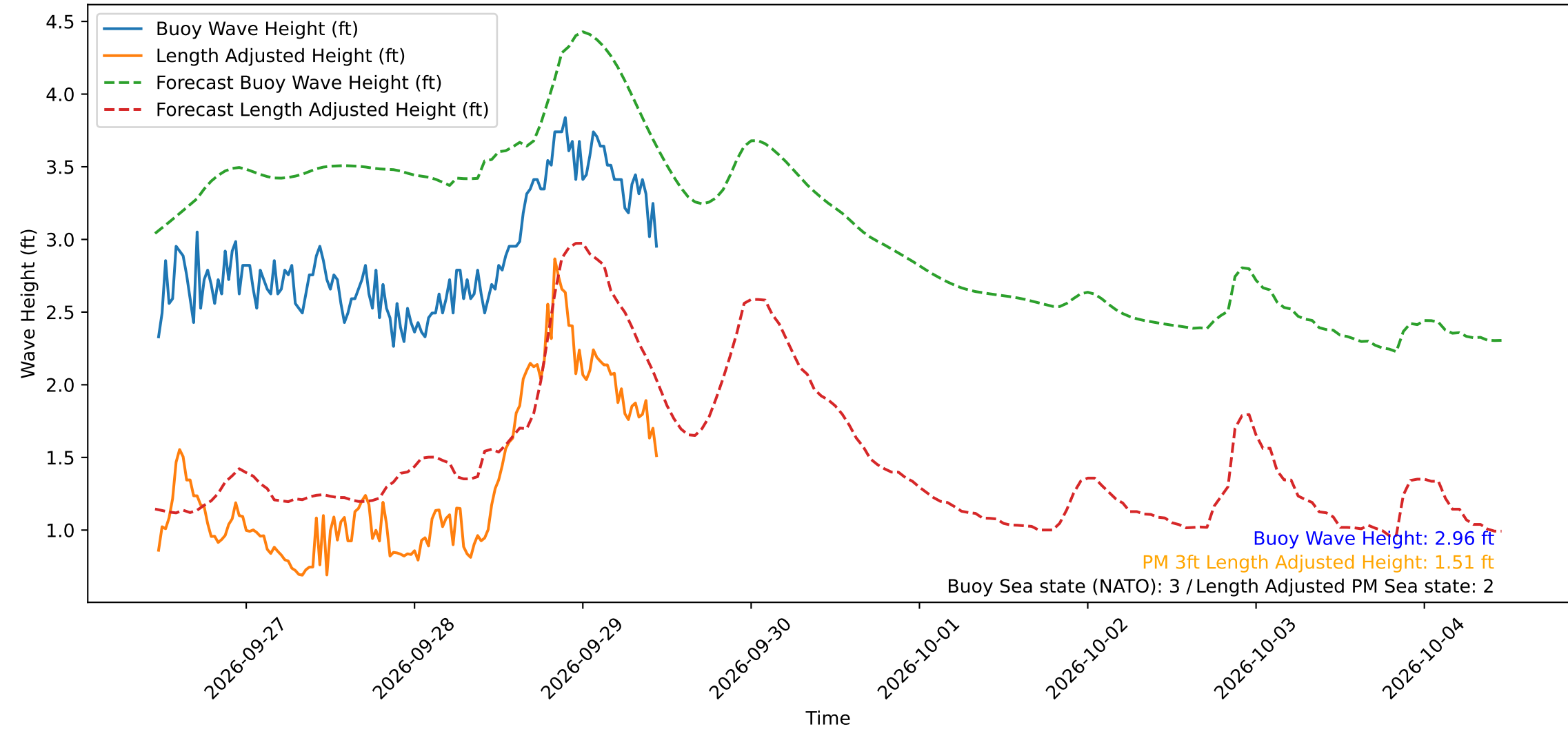
Wave Heights over Time for Red Beach at 2026-09-29 11:20:51
