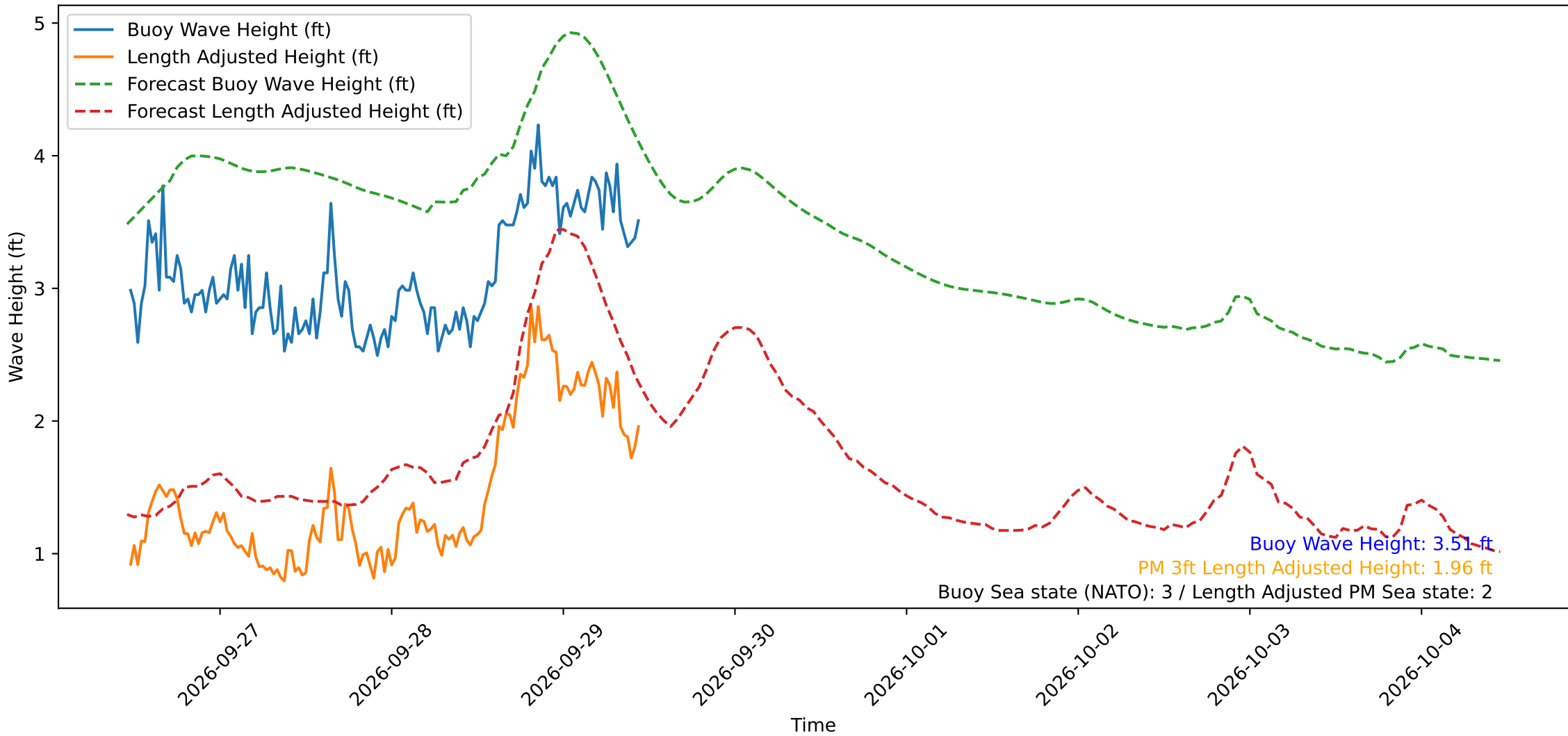
Wave Heights over Time for Oceanside Harbor at 2026-09-29 11:20:30
