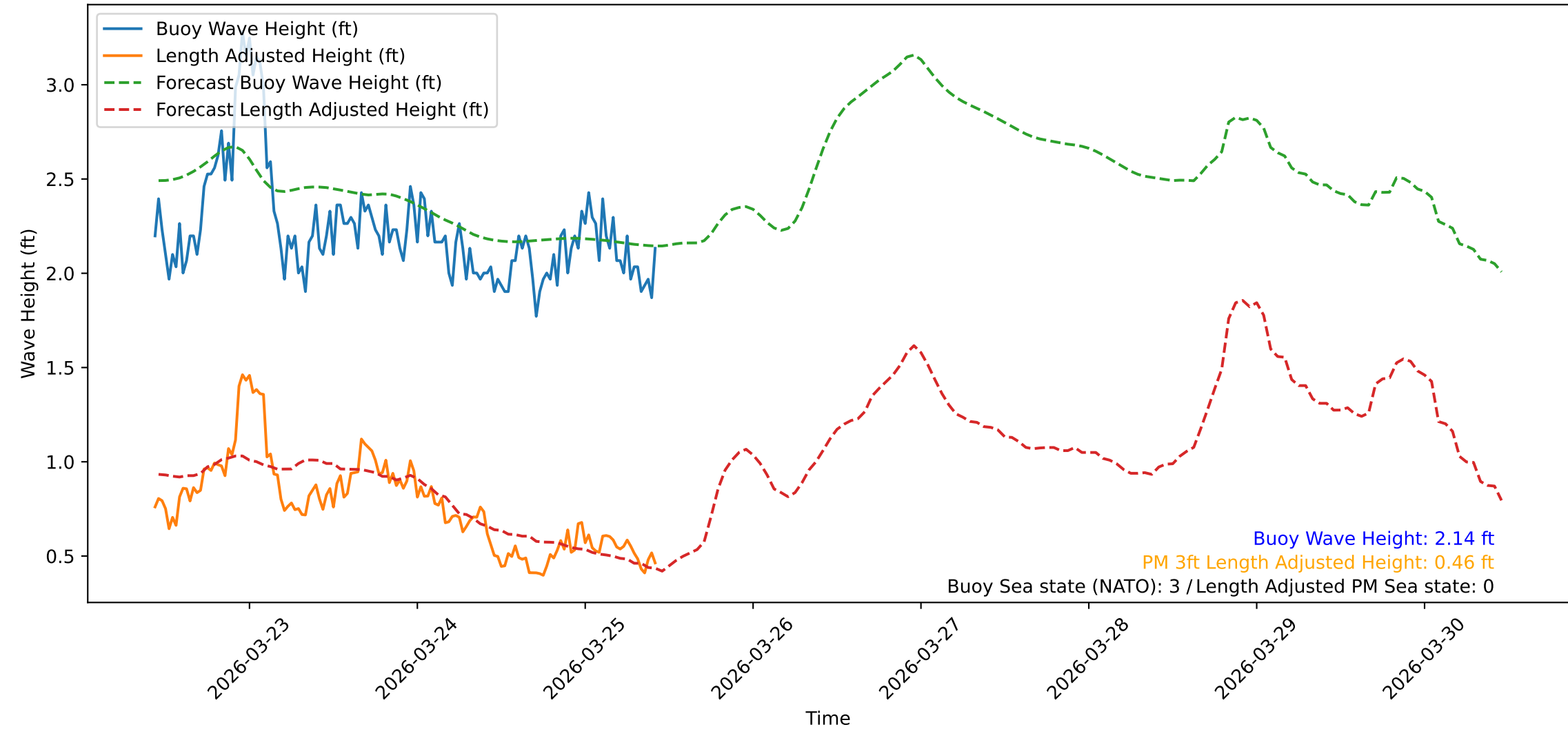
Wave Heights over Time for Green Beach at 2026-03-25 10:41:09
